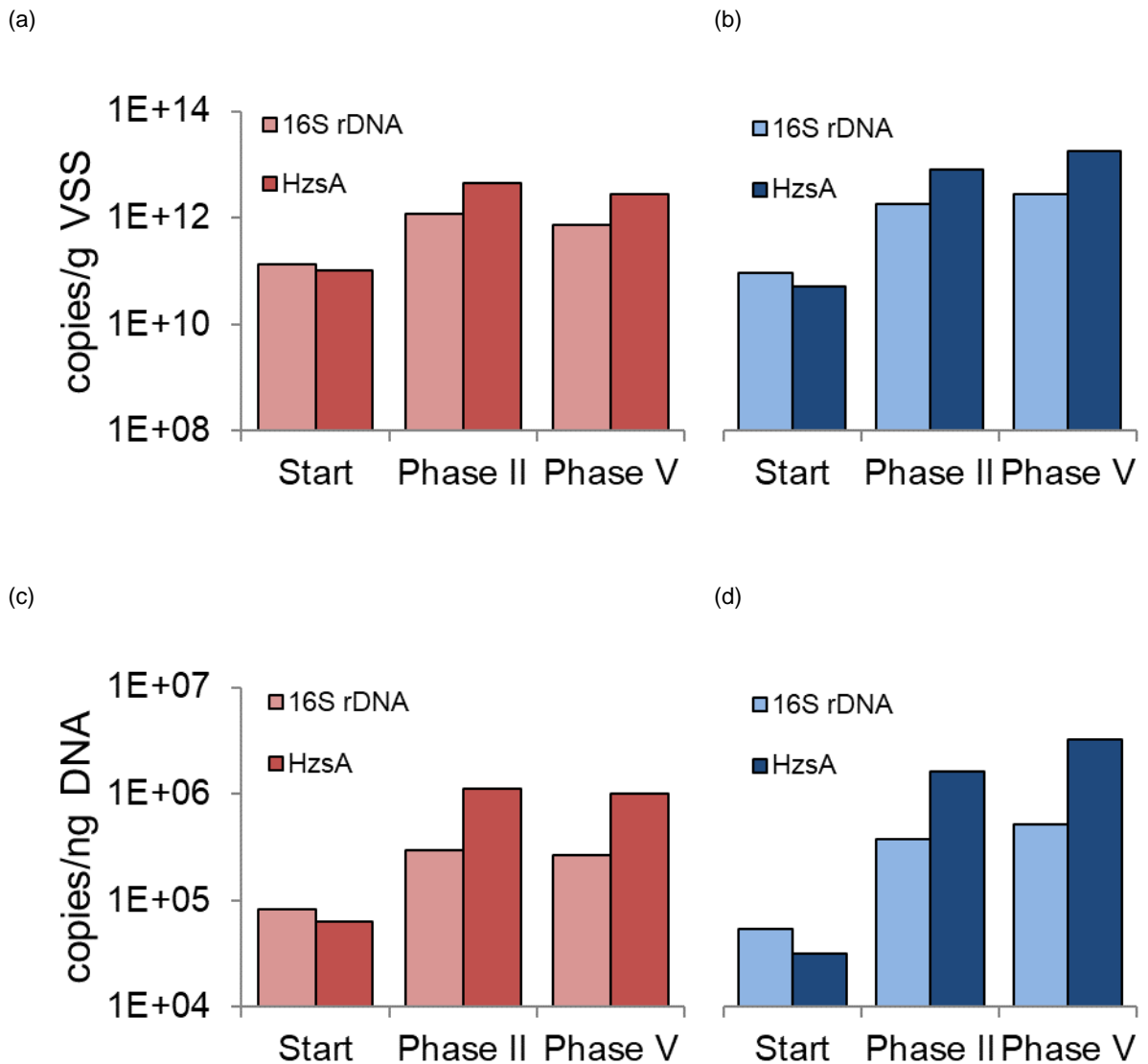
Figure 3.4 - Evolution of overall AnAOB abundance as determined by qPCR analyses based on AnAOB 16S rDNA (lighter bars) and the HzsA functional gene (darker bars). Top row shows the data expressed per g of VSS for SBR constantT (a) and SBR loweringT (b). Bottom rows show the same data expressed per ng of DNA for SBR constantT (c) and SBR loweringT (d). The corresponding sampling times for Start, Phase II and Phase V are 10, 134 and 293 days, respectively.
