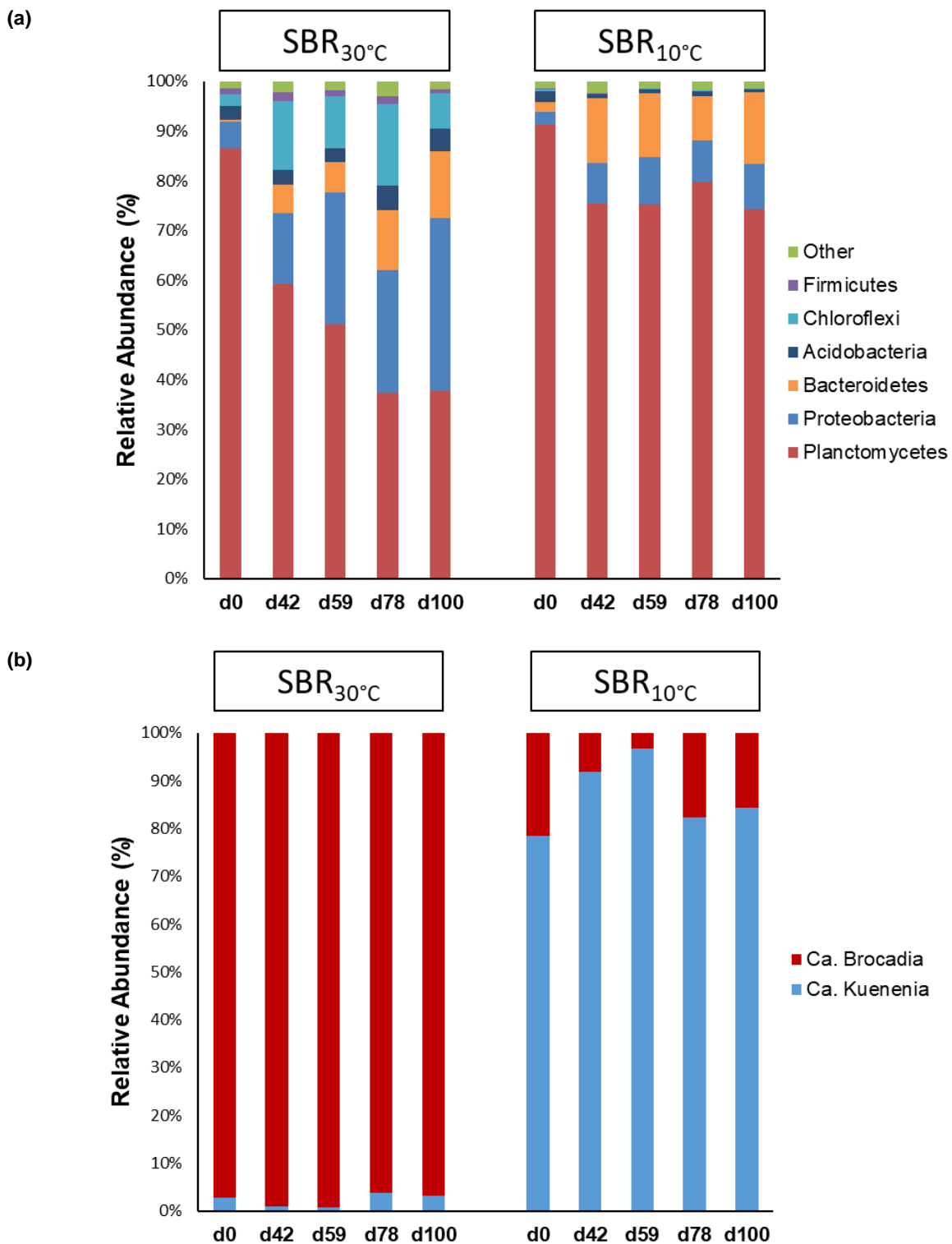
Figure 4.4 – Evolution of (a) Microbial community at Phylum level. and (b) anammox diversity at genus level throughout the experiment (abscissa represents operating days) in SBR 30°C (left) and SBR 10°C (right)
