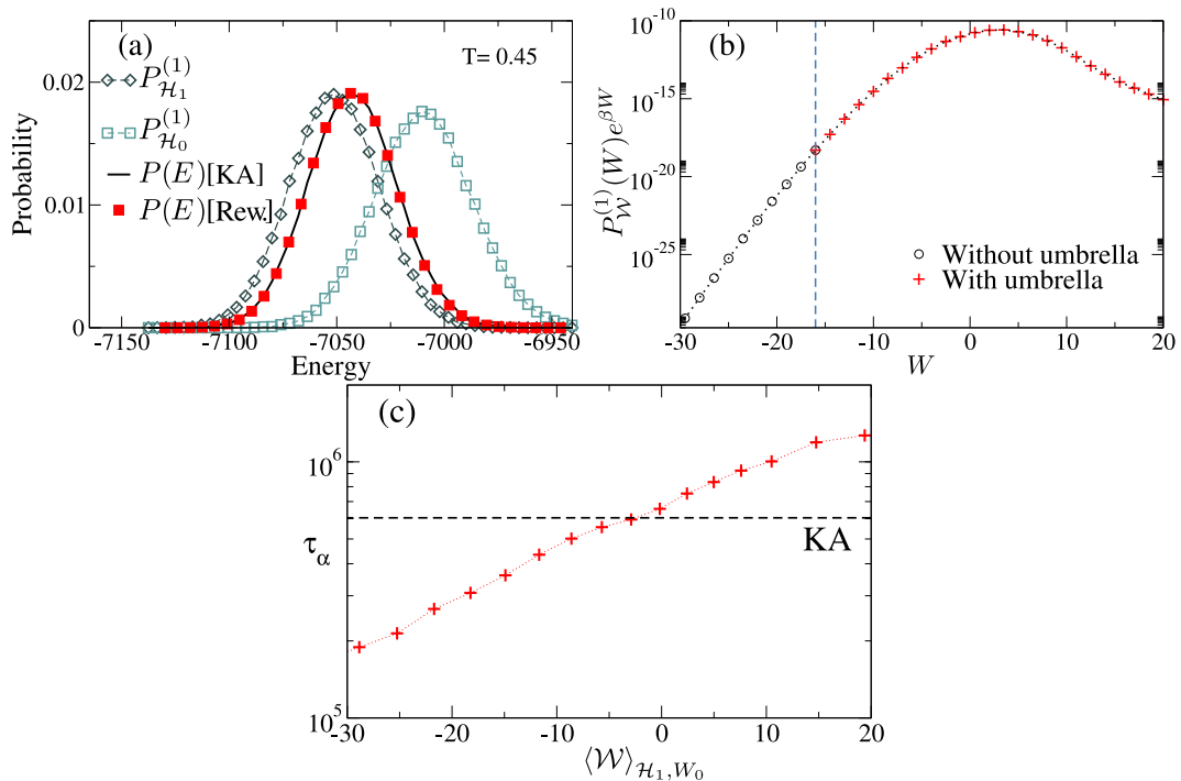
FIG. VII.1 | (a) Probability distributions P_{\mathcal{H}_1}^{(1)} , P_{\mathcal{H}_0}^{(1)} of energies \mathcal{H}_1 and \mathcal{H}_0 in the extended Kob-Andersen (KA 1 ) system at T = 0.45 along with the reweighted probability distribution P(E) [Rew.] of the energy for the Kob-Andersen (KA) model which is obtained from Eq. (VII.7). The probability distribution P(E) has also been directly measured in the KA model [KA] to check the quality of the reweighting procedure. (b) Plot of P_{\mathcal{W}}^{(1)}(W)e^{\beta W} with (red) and without (black) umbrella sampling. The vertical dashed line marks the limit of \mathcal{W} in the unbiased Monte Carlo simulations of the KA 1 model. (c) Relaxation time \tau_\alpha of the system in the different umbrella simulations as a function of \langle \mathcal{W} \rangle_{\mathcal{H}_1, \mathcal{W}_0} , the average value of \mathcal{W} .
