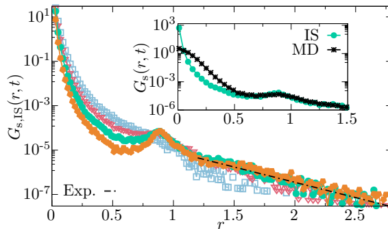
FIG. VI.4 | van Hove distribution of displacements in the inherent structures G_{s,IS}(r,t) when \hat{\Delta}_{IS}(t) = 1.5 \times 10^{-2} . The dashed-dotted line is an exponential fit of the tail of the distribution. The inset shows a comparison of the van Hove distribution in the normal dynamics (MD) and in the inherent structures (IS) for T = 0.07 . They agree at large displacements but the peak at r = 0 is significantly narrower and higher in the inherent structures because thermal vibrations are partially filtered. The color code is given in FIG. VI.1 (a).
