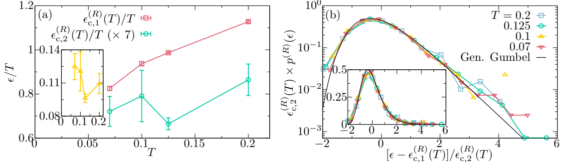
FIG. V.5 | (a) Average \epsilon_{c,1}^{(R)}(T) and standard deviation \epsilon_{c,2}^{(R)}(T) of the localising field for several temperatures which range from the experimental glass transition temperature to the onset temperature of glassy behaviour and for the case T = T_0 . Both quantities have been divided by the temperature (the Boltzmann constant is set to unity). The standard deviation has been multiplied by 7 in order to cover a similar range as the first moment. Errorbars are computed thanks to the jackknife method when the average over the reference configurations is performed [294], they are too small to be seen for the first cumulant. The inset represents the ratio of the standard deviation to the average localising field, namely, \epsilon_{c,2}^{(R)}(T)/\epsilon_{c,1}^{(R)}(T) , with respect to the temperature T . (b) Histograms p^{(R)}(\epsilon) of the localising field for the case T = T_0 . The data have been rescaled by \epsilon_{c,2}^{(R)}(T) and plotted as a function of [\epsilon - \epsilon_{c,1}^{(R)}(T)]/\epsilon_{c,2}^{(R)}(T) , see Eq. (V.13). They follow a master curve which is well fitted by a generalised Gumbel distribution with a single adjustable parameter \alpha \simeq 1.3 , see Eq. (V.14).
