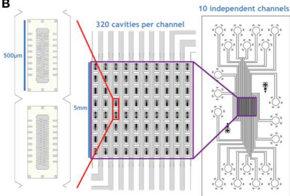
Figure 7.3 The high-throughput and 10 independent channel-optimization design allowing to monitor more conditions within one experiment
