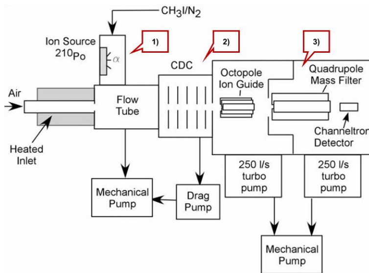
Figure I-4 Schematic of CIMS for \text{NO}_3 radicals measurement [25].
