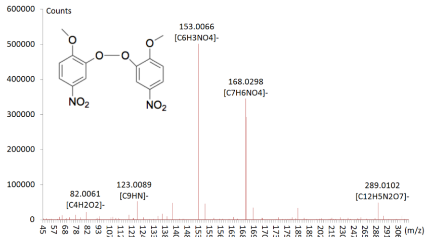
Figure S8 LC/MS/MS product ion spectra of m/z 335 compound: association of 2 nitroguaiacols at RT = 14.26 min (Fig.IV-10).
