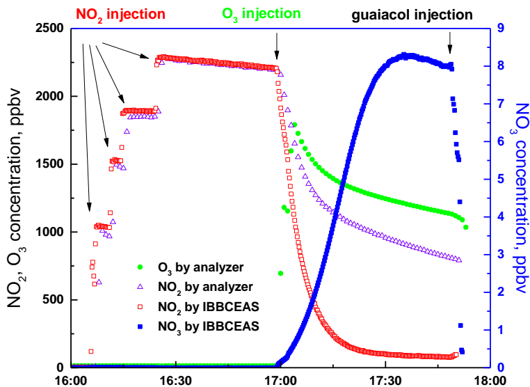
Figure IV-6 Time series of NO 2 , O 3 and NO 3 in experiment of NO 3 + guaiacol.
