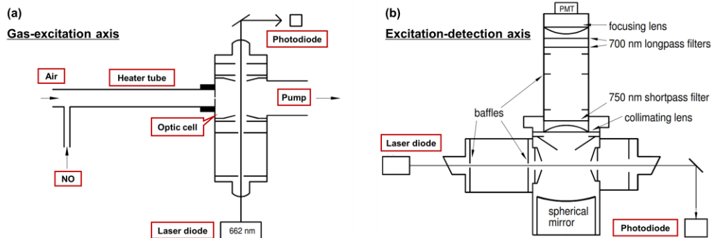
Figure I-6 LIF instrument for \text{NO}_3 measurement [35]: (a) Top view; (b) Right view.
