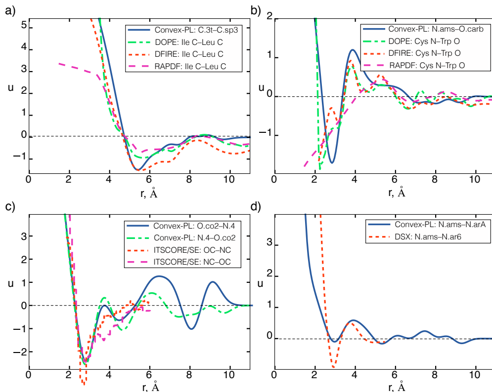
Figure 2.4: Comparison of the Convex-PL potentials with DOPE, DFIRE and RAPDF potentials for protein-protein interactions (a-b), with ITSCORE/SE (c) and with DSX (d) potentials for protein-ligand interactions. For the protein-ligand potentials, the two atom types in a pair correspond to the protein and ligand atoms, respectively. All the reference potentials' values were adapted from the plots found in the literature. The following interactions are plotted, a) sp3 carbon with sp3 carbon; b) secondary amide nitrogen with amide oxygen; c) negatively charged oxygen with positively charged nitrogen and vice versa; d) secondary amide nitrogen with aromatic nitrogen.
