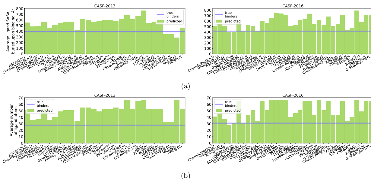
Figure 1.2: Statistics for the CASF 2013 and 2016 benchmarks. (a)-(b) The purple line represents the average values of buried SASAs and numbers of atoms computed for ligands that natively bind target proteins and should have been predicted as the most affine binders [1] . The green boxes correspond to decoys that were top-ranked by scoring functions assessed on the virtual screening test from the CASF benchmarks 2013 and 2016. The scoring functions are sorted by the ability to predict the highest affinity binder in the 5% of the top-ranked decoys. SASA values were computed with PyMOL's[96] get_area() function with dot_solvent set to 3.
