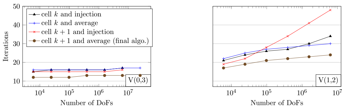
Figure 3.11 Scalability comparison of different versions of the algorithm, applied on the 2D homogeneous problem discretized with the structured triangular mesh for k = 1 . On the left, the V(0,3) cycle is used, on the right, V(1,2) . The various option combinations are labeled according to Table 3.1.
