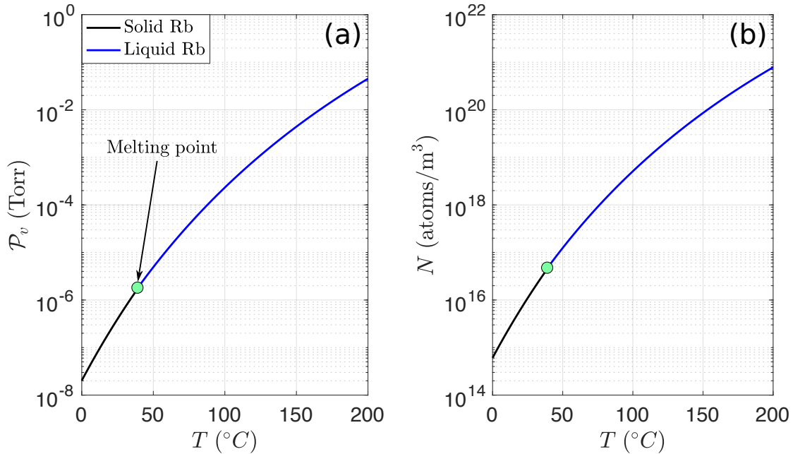
Figure 3.5: Vapor pressure (a) and atomic density (b) as function of the temperature T . The melting point of rubidium is 39.31^\circ\text{C} . The density is in \text{atoms}/\text{m}^3 .
