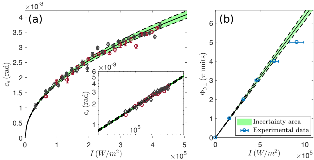
Figure 4.12: (a): Speed of sound c_s as function of the pump intensity \mathcal{I}_0 . The red circles and the grey diamonds represent two sets of data taken successively at the same laser detuning and vapor temperature. The sound velocity increases with the square root of \mathcal{I}_0 , as expected. The theoretical prediction (black line) matches the data pretty well. No free-parameter is needed because the nonlinear refractive index n_2 has been measured independently, using the ring counting technique of subsection 2.3.2. The uncertainty on c_s (green area) derives from the uncertainty on n_2 . (b): Ring-counting measurement. The self-phase \Phi_{\text{NL}} accumulated by a Gaussian beam propagating through the cell is measured as function of the beam intensity. The nonlinear refractive index is obtained by fitting the data with a line. We find n_2 = 3.3 \pm 0.2 \times 10^{-11} \text{ m}^2/\text{W} .
