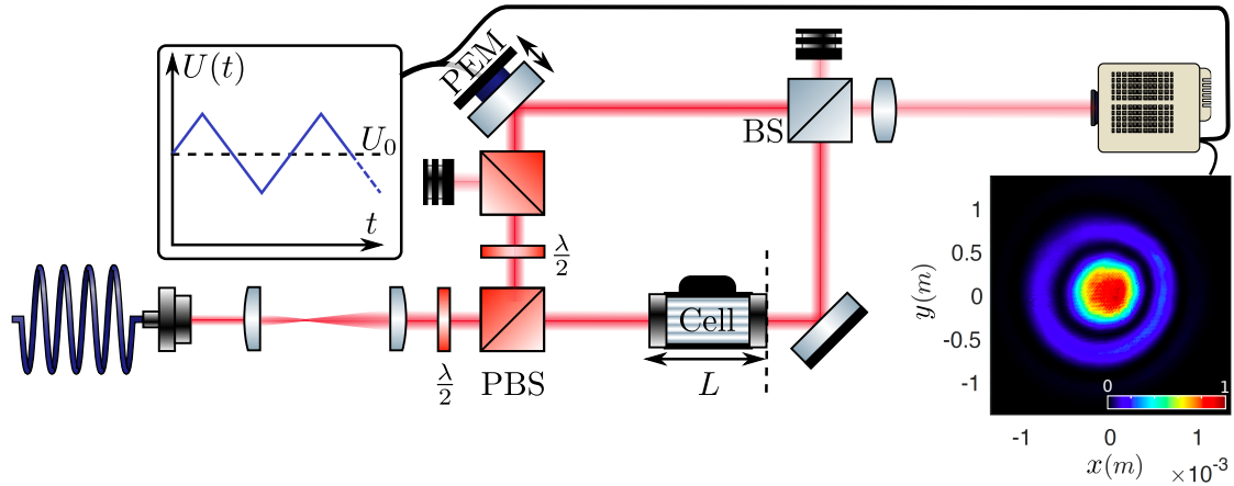
Figure 3.12: Experimental setup. A Mach-Zehnder interferometer is used so as to measure the beam transverse phase profile in the cell exit plane. Left inset: high voltage triangular signal making the PEM scan the phase of the reference beam. Right inset: example of an interferogram obtained when the angle between the reference and the fluid is zero.
