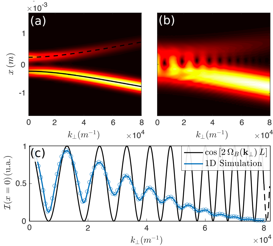
Figure 4.15: Envelope of the intensity profile along x in the output plane as function of k_{\perp} , for a probe width w_{0,x} of 150 \mu\text{m} (a) and 450 \mu\text{m} (b) respectively. In figure (a), the envelopes of the wave-packets are fully separated in the cell exit plane. This is not anymore the case on figure (b). Interference between the upward- and downward-moving wave-packets occurs in that case. Depending on the probe wave-vector, the envelope of the density modulation exhibits two distinct peaks (destructive interference) or just one (constructive interference). Figure (c) shows the intensity at x = 0 in the exit plane as function of k_{\perp} for w_{0,x} = 450 \mu\text{m} . It oscillates in a similar way as \cos[2\Omega_B(k_{\perp})L] (black solid line), that describes the beating between two counter-propagating Bogoliubov modes at k_{\perp} . The amplitude of the oscillations is damped because the overlap between the wave-packets decreases with k_{\perp} . Parameters: \Delta n = 1.0 \times 10^{-5} , L = 7.5 \text{ cm} and \alpha = 0 .
