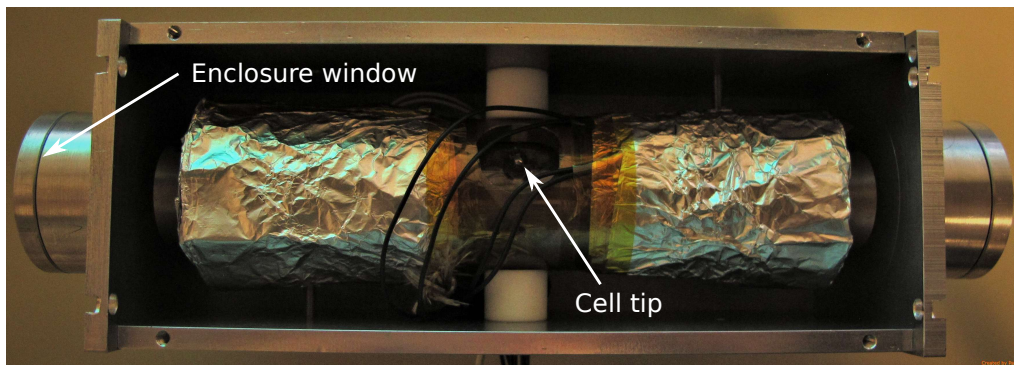
Figure 3.1: Heating system. A 7.5 cm long cell is placed inside 5 mm thick copper cylinder. Flexible heaters are arranged all around and covered with several layers of aluminum foils to reduce losses by thermal radiation and provide a better heating efficiency. The cell tip (visible at the center of the picture) is about 80^\circ\text{C} .
