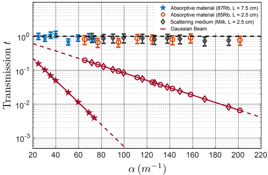
Figure 5.15: Measure of the on-axis transmission t of the Bessel beam as a function of the attenuation coefficient \alpha . Data obtained with the rubidium vapors have been plotted in blue stars ( ^{87}\text{Rb} ) and orange circles ( ^{85}\text{Rb} ). Data obtained with the water-milk mixture have been plotted in grey diamonds. The two red lines show the transmission expected from the Beer-Lambert law through a 2.5 cm and a 7.5 cm long lossy material
