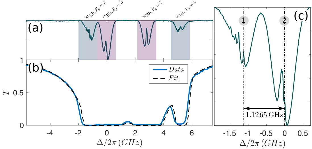
Figure 3.4: (a) and (c): Saturated absorption spectra obtained using an isotopic mixture of rubidium atoms (natural proportions), heated up at 50^\circ\text{C} to increase the atomic density and the signal over noise ratio. As mentioned in the text, the F_g = 3 \rightarrow F_e = 4 transition peak (2) has been chosen as origin for the x -axis; the frequency scale has been calibrated using the frequency spacing between peaks (2) and (1), the latter corresponding to the F_g = 2 \rightarrow F_e = 3 transition. (b) Transmission spectrum of an isotopically pure ^{85}\text{Rb} vapor heated up at 134^\circ\text{C} . The experimental profile (blue line) has been fitted to extract the absolute vapor temperature (dashed line). The cell is 7.5 cm long.
