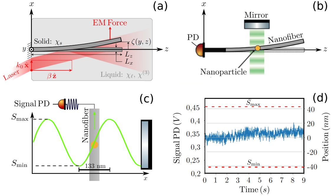
Figure 6.8: Optomechanical signature of superfluidity. (a): Sketch of the experimental setup proposed by Larré et al. in [100]. The left end of the obstacle is clamped to the cell entrance window and its right end is free to move. Initially, the obstacle is aligned along the z -axis. When the laser is switched on, the obstacle bends under the radiation pressure. The position \zeta(x, L_z) of the right tip increases with the fluid intensity \mathcal{I}_f before dropping to zero when passing through the normal/superfluid transition. (b) and (c): Displacement measurement. A gold nanoparticle is dropped onto a nanofiber (obstacle). A standing-wave is created by reflecting a laser beam on a mirror. The nanoparticle diffuses more or less light into the fiber depending on its position inside this standing-wave. By collecting the scattered light with a photo-diode (PD), we can measure \zeta(x, L_z) with an accuracy of \pm 20 nm (see figure (d)).
