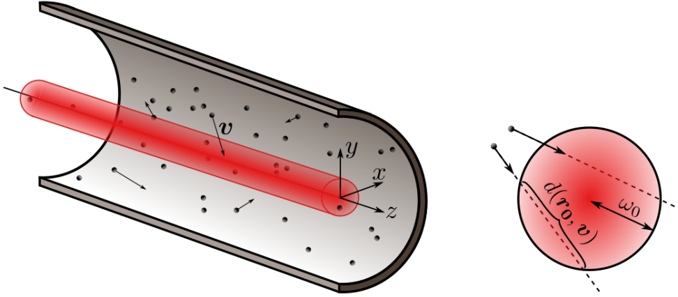
Figure 1.6: Left: sketch of the beam propagation inside the vapor cell. Right: beam cross-section at a given position z on the optical axis. The time an atom takes to flight across the laser beam depends on its position \mathbf{r}_0 and velocity \mathbf{v} when it enters the interaction region.
