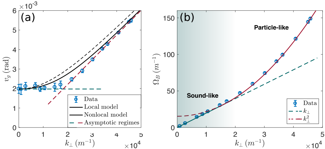
Figure 4.11: (a): Group velocity v_g as function of the transverse wave-vector k_{\perp} = k_0 \sin(\theta_i) . The blue circles represent the experimental data obtained for a fluid power \mathcal{P}_f = 175 \text{ mW} . The theoretical model is plotted in black solid. It takes into account the nonlocal response of the vapor, due to the ballistic transport of fast moving excited atoms. For comparison, the group velocity predicted by the local theory is plotted in black dashed on the same graph. The dashed lines highlight the asymptotic behaviours of the group velocity, which remains constant in the sonic regime (cyan) and linearly increase in the particle-like regime (red). (b) shows the dispersion relation obtained after integration of the group velocity in (a). It exhibits a linear increase at low k_{\perp} characterized by the sound velocity c_{s,\text{eff}} .
