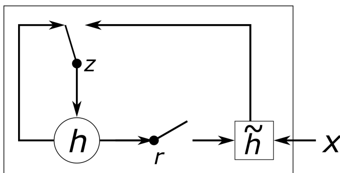
Figure 2.3: Illustration of the GRU showing the flow of information between input/output and the control gates. \mathbf{h} is the hidden state, \mathbf{r} the reset gate, \mathbf{z} the memory gate and \tilde{\mathbf{h}}^t the candidate hidden state. The illustration is taken from [9].
