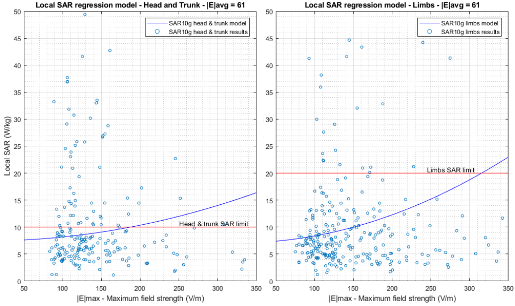
Figure 5.5: Local SAR regression models (solid lines) and local SAR simulation results (circles) versus E_{max} . Head & trunk local SAR on left figure, limbs local SAR on the right figure. Results are shown for E_{avg} = 61 V/m.
