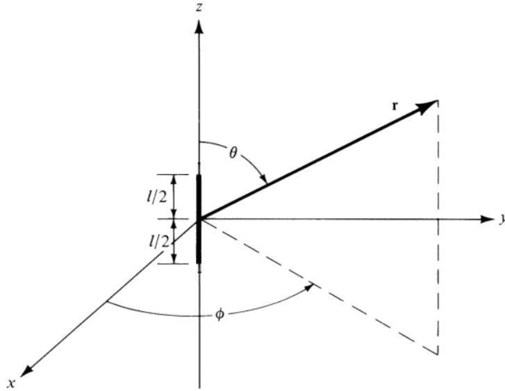
Figure 3.2: Infinitesimal dipole in the initial state [Bal16].
