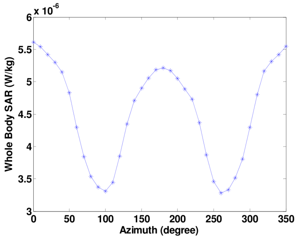
Figure 2.4: Whole-body averaged SAR for an incident single plane wave and a 10 deg azimuth angle step [KCH + 11a].
