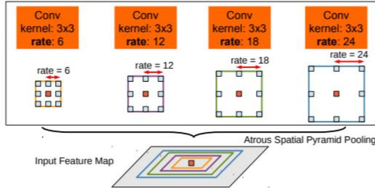
FIGURE 2.2: Atrous Spatial Pyramid Pooling uses dilated convolutions with increasing dilation rates to extract multi-scale contextual information.
