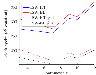
Figure 3.5: CRV d^2 const. ( \lambda = 8 ).
