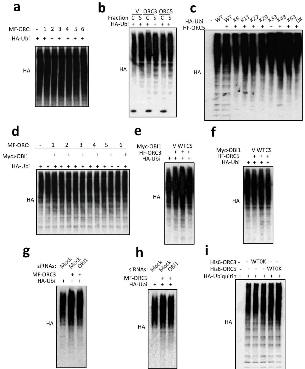
Supplementary Figure 7: Characterization of ORC ubiquitylation; complementary to Figure 3-5 a-c , Expression of HA-tagged ubiquitin in the experiments described in Figure 3a-c was evaluated by western blotting of input extracts. d-h , Expression of HA-tagged ubiquitin in the experiments described in Figure 4a-e was evaluated by western blotting of input extracts. i , Expression of HA-tagged ubiquitin in the experiment described in Figure 5a was evaluated by western blotting of input extracts.
