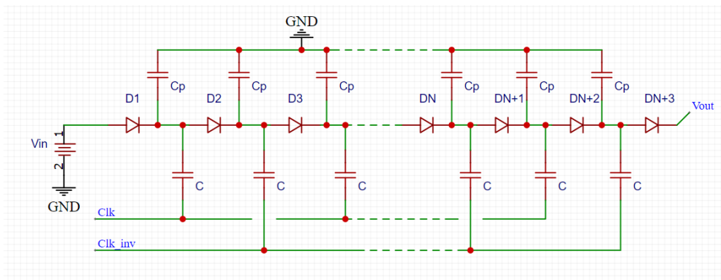
FIGURE 50 – Structure originale de Dickson
