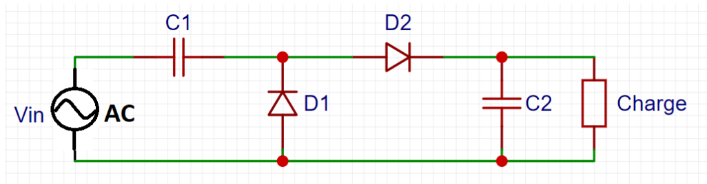
FIGURE 48 – Structure de Greinacher, Cockcroft et Walton 48
