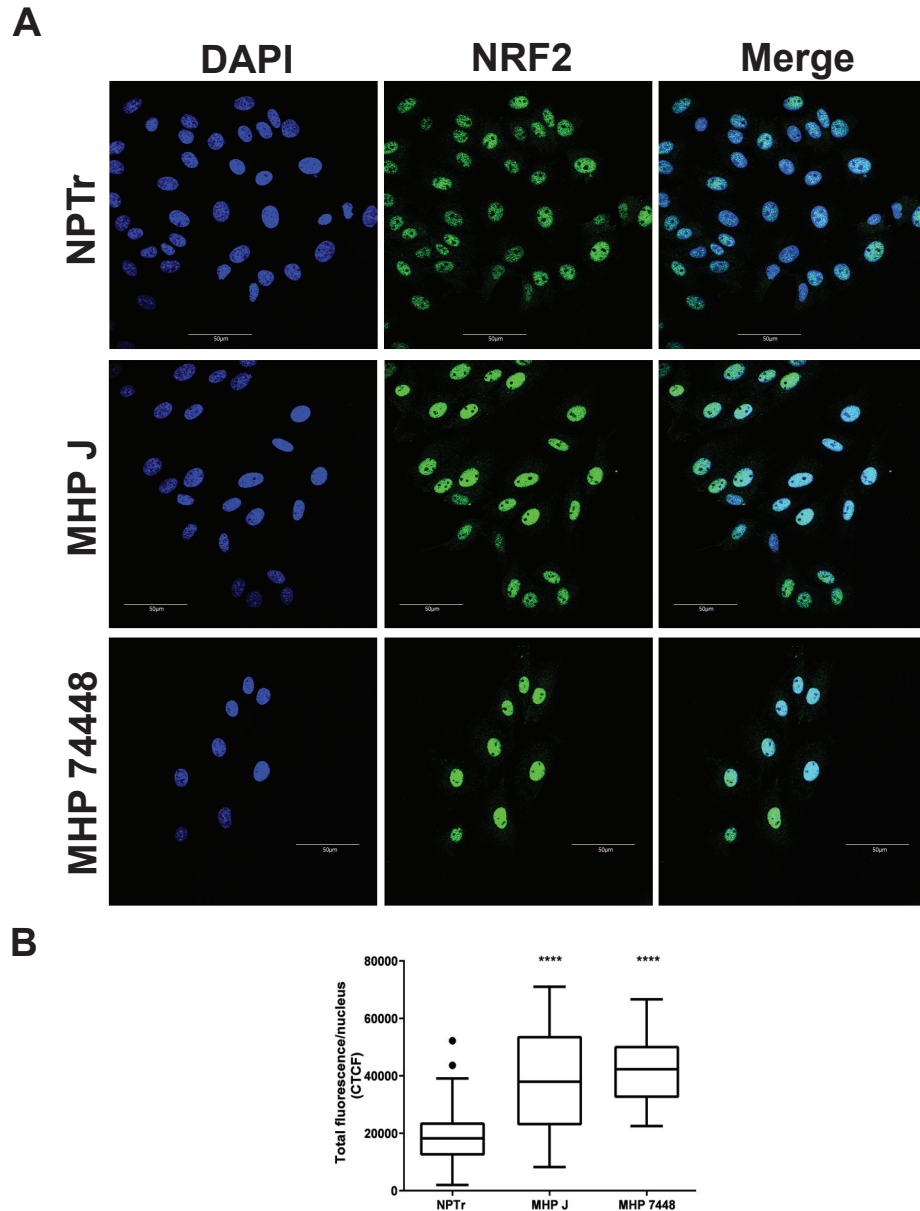
Figure 2.7 – Localization and expression pattern of the NRF2 protein in cells infected with M. hyopneumoniae . A . Results of the immunofluorescence microscopy analysis indicating the accumulation of NRF2 in the nuclei of infected cells after 1 h of incubation. Both attenuated (J) and virulent (7448) strains of M. hyopneumoniae induced the accumulation of the transcription factor in the nuclei of the epithelial cells. Eukaryotic cell NRF2 was labeled with anti-NRF2 antibody (green) and nuclei were stained with DAPI (blue). Scale bars: 50 \mu\text{m} . B . Total NRF2 green fluorescence per nucleus of control and infected cells. Both M. hyopneumoniae strains significantly increased the concentration of NRF2 in the nuclei of infected cells. Box-plots represent the measures of at least 25 nuclei in each condition. Outliers are represented as black dots. CTCF - corrected total cell fluorescence. NPTr - uninfected cells. MHP J - NPTr cells infected with M. hyopneumoniae strain J. MHP 7448 - NPTr cells infected with M. hyopneumoniae strain 7448. **** p < 0.0001
