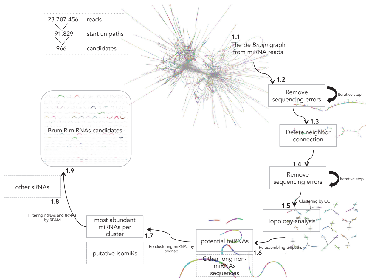
Figure 3.7 – BRUMIR algorithm. Different steps of BRUMIR to discover miRNAs from sRNA-seq data. 1.1 De Bruijn graph step, 1.2 Tips removal iterative step, 1.3 Delete neighbor connection step, 1.4 Tips removal step repetition, 1.5 Topology analysis step, 1.6 Re-assembling unipaths by CC step, 1.7 Re-clustering by overlap step, 1.8 Filtering other sRNAs by RFAM step, 1.9 BRUMIR candidates catalog.
