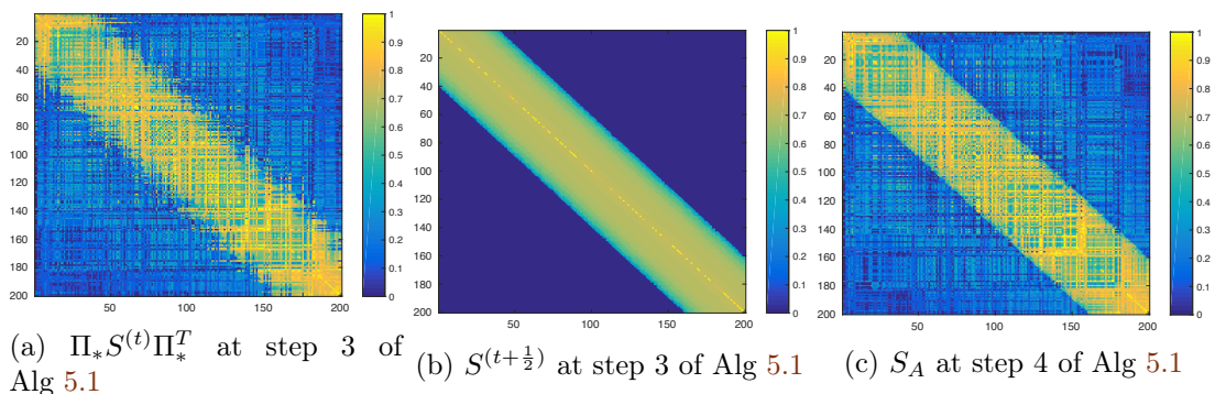
Figure D.4: Three steps of Algorithm 5.1 for a sparse matrix S with parameters n = 200 , \delta = 40 , s = 0 , N/n = 4 .
