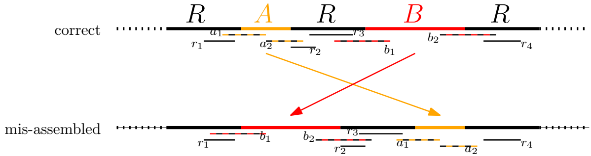
Figure 1.6: Genome rearrangement around a repeat that occurs in three places. The reads at the junction between one of the two sequences A , B and a repeat R have apparent overlaps with the two other repeats, resulting in two possible layouts consistent with the overlaps constraints (the correct and the mis-assembled).
