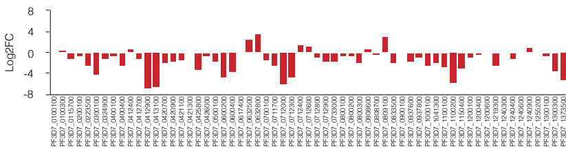
Differential var expression CRISPRi vs Control
