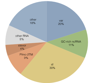
Top down regulated genes
