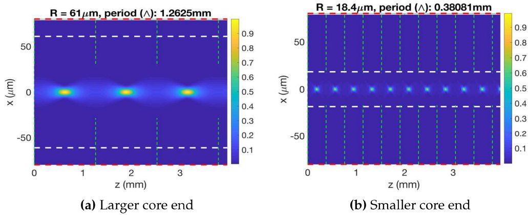
Figure 2.6: Self-imaging phenomena in GRIN MMF: (a) Core radius 61 \mu\text{m} (b) Core radius 18.4 \mu\text{m}
