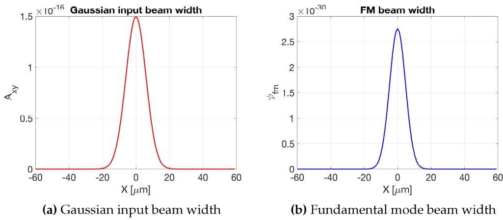
Figure 2.5: Gaussian input beam diameter of 10\mu\text{m} FWHM and fundamental mode width.
