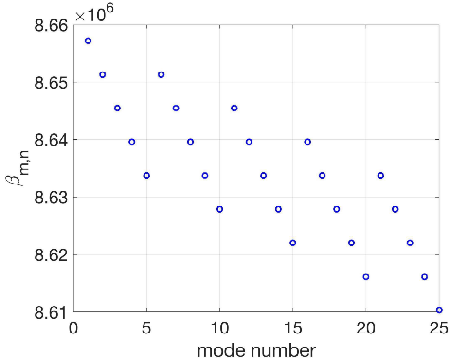
Figure 2.3: Graded-index multimode fiber propagation constant plot.
