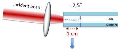
Figure 2.7: Inclined input beam injected at the input facet of graded-index MMF.
