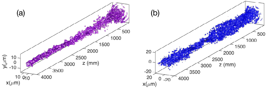
Figure 6.17: (a) Beam cleaning in a nonlinear Yb-doped GRIN fiber. Forward pump of 20W; input signal maximum intensity 0.5 \text{ GW/cm}^2 . (b) The same as in panel (a), but without Kerr nonlinearity n_{2kerr} = 0 .
