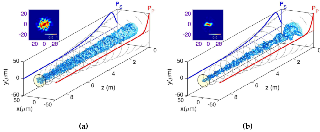
Figure 6.21: Signal power propagation in multimode tapered fiber: (a) Iso-intensity surface at half width of maximum intensity in a Yb-doped active taper fiber in the absence of Kerr effect ( n_{2\text{kerr}} = 0 ). The blue (red) curve reproduces the qualitative evolution of the signal (pump) power. The grey circles show the local size of the fiber core. The inset shows the output beam pattern. (b) The same as in figure 6.21a, but here in the presence of Kerr nonlinear effect ( n_{2\text{kerr}} \neq 0 )
