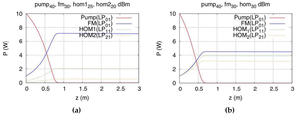
Figure 3.3: Amplification of signal power along fiber length: (a) Higher fundamental modes ( LP_{01} ) power than high order modes (b) Power of fundamental mode ( LP_{01} ) the same as other high-order modes ( LP_{11} , and LP_{21} )
