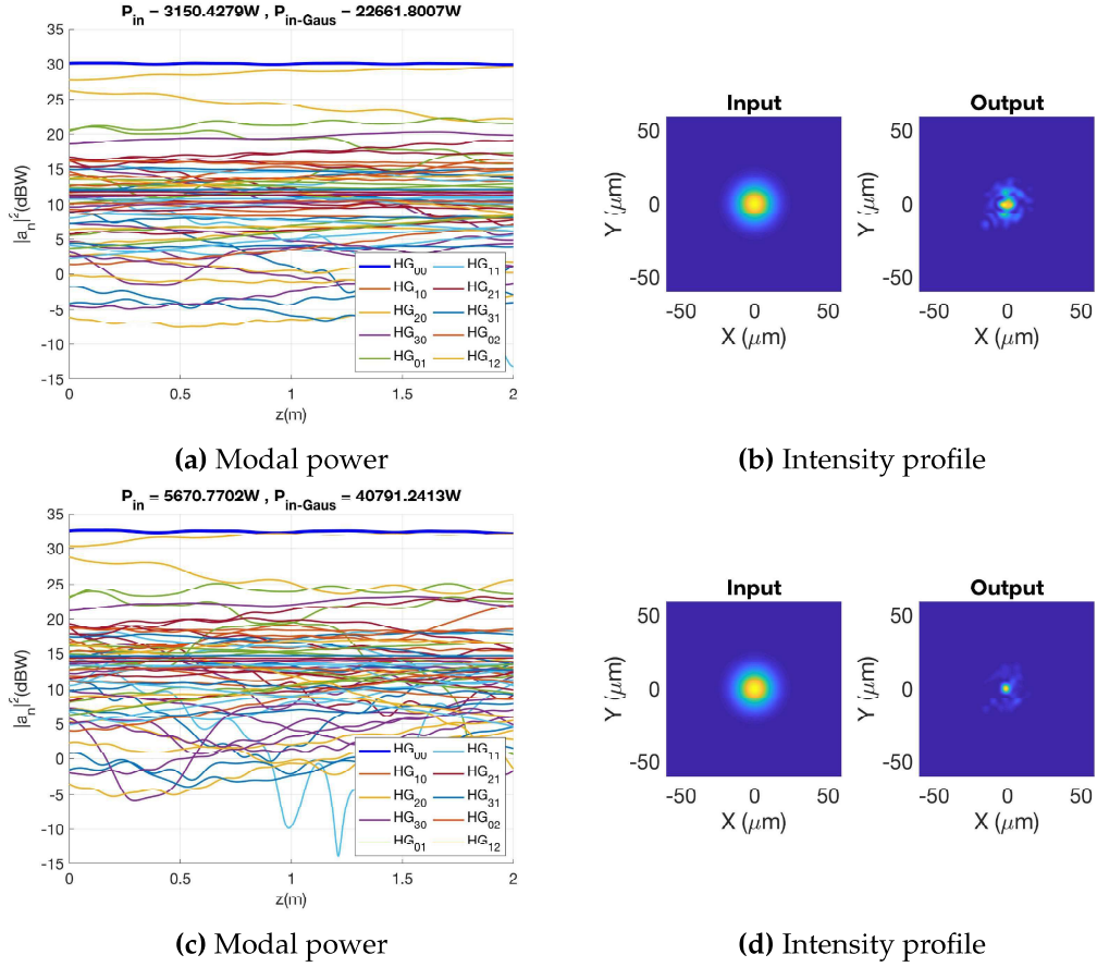
Figure 5.16: Modal power and intensity profiles with Kerr at higher input power
