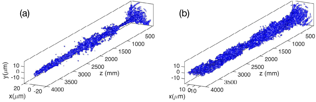
Figure 6.14: Beam cleaning in a nonlinear GRIN fiber. (a) Input signal maximum intensity 5\text{GW}/\text{cm}^2 . (b) The same as (a), but with input signal maximum intensity 0.5\text{GW}/\text{cm}^2 .
