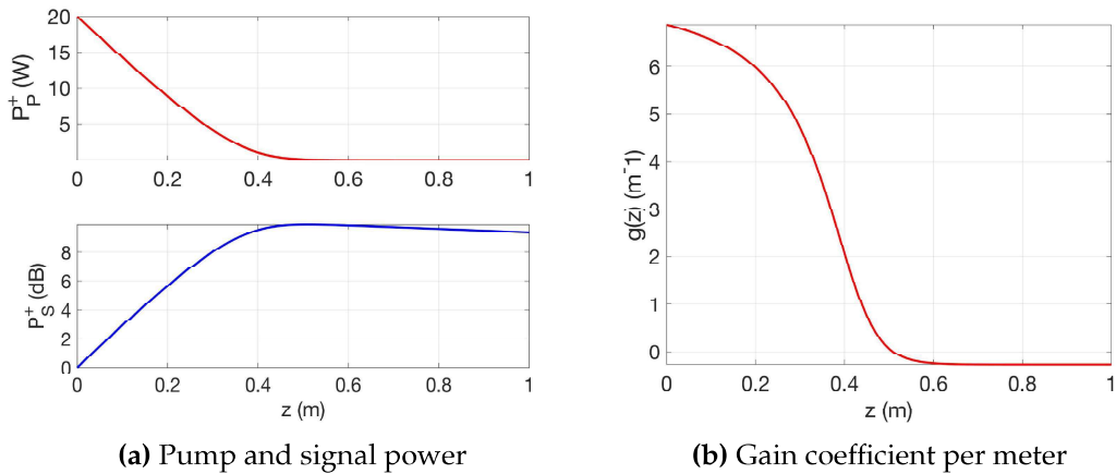
Figure 4.10: Forward pump and signal power propagation with 75\mu\text{m} signal diameter.
