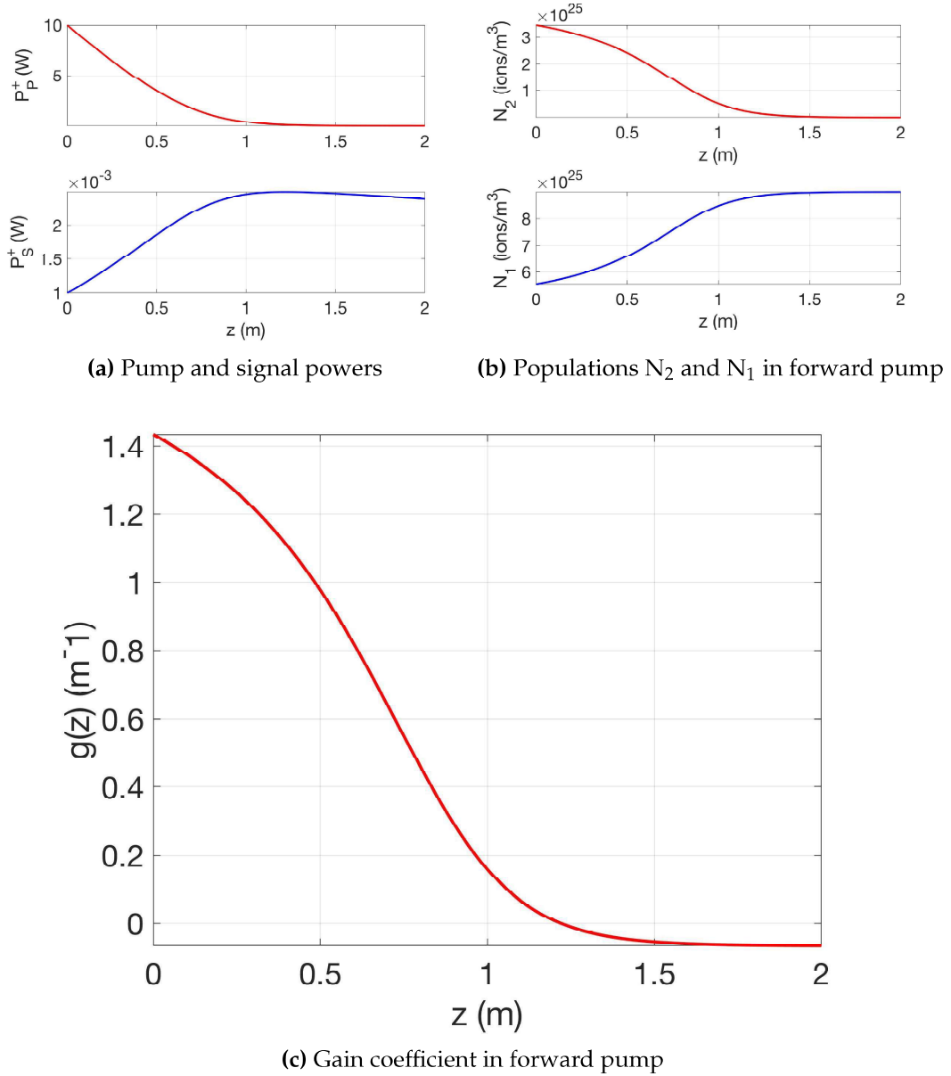
Figure 4.4: Signals, population and gain coefficient in forward pumping.
