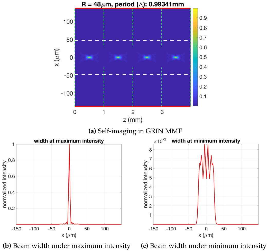
Figure 4.7: Local intensity saturation phenomenon in GRIN MMF
