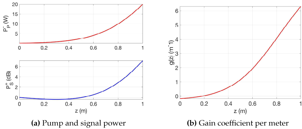
Figure 4.9: Backward pump and signal power propagation with 75\mu\text{m} signal diameter.
