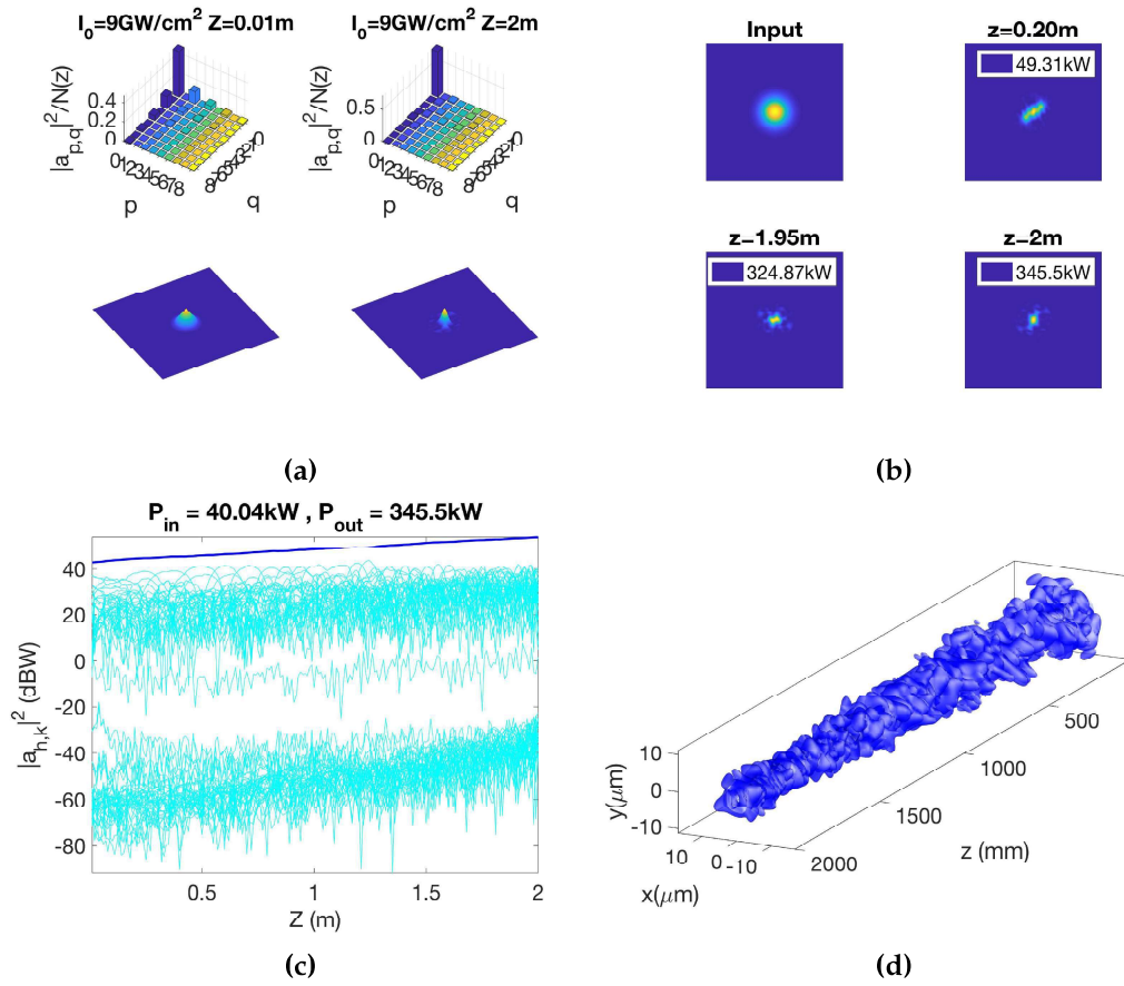
Figure 6.10: Kerr, gain and disorder without saturation: (a) Fractional power of modes at beginning and end of fiber length (b) Intensity profile plot of input and output guided modes (c) Fractional power evolution of modes (d) Iso-intensity plot across fiber length
