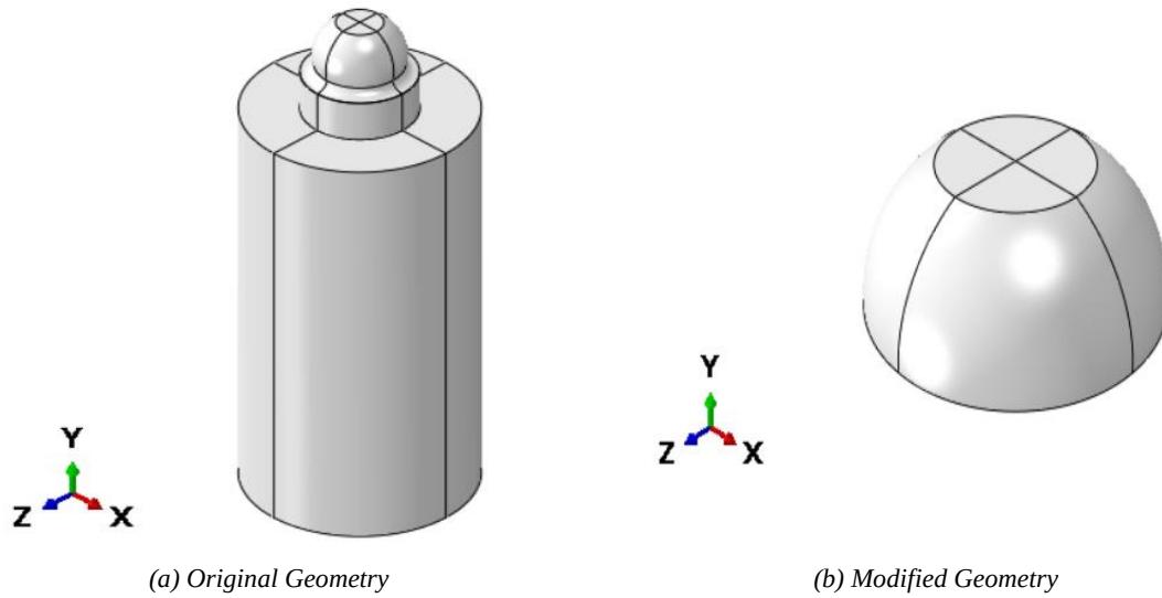
Figure 5-30: Impact geometry used in dynamic impact numerical simulation.
