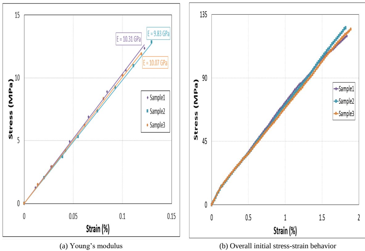
Figure 3-5: Mechanical performance of the composite star sample.
