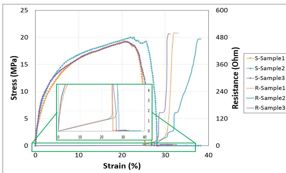
Figure 2-14: Overall electromechanical response of CM sensor specimens.
