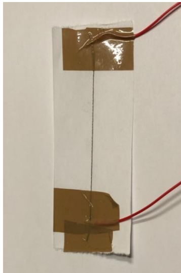
(a) Sensor I: Nylon/Ag fiber sensor
