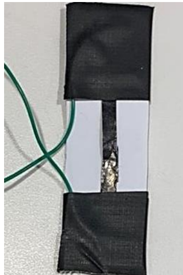
(b) Sensor II: Conductive membrane (CM) sensor
