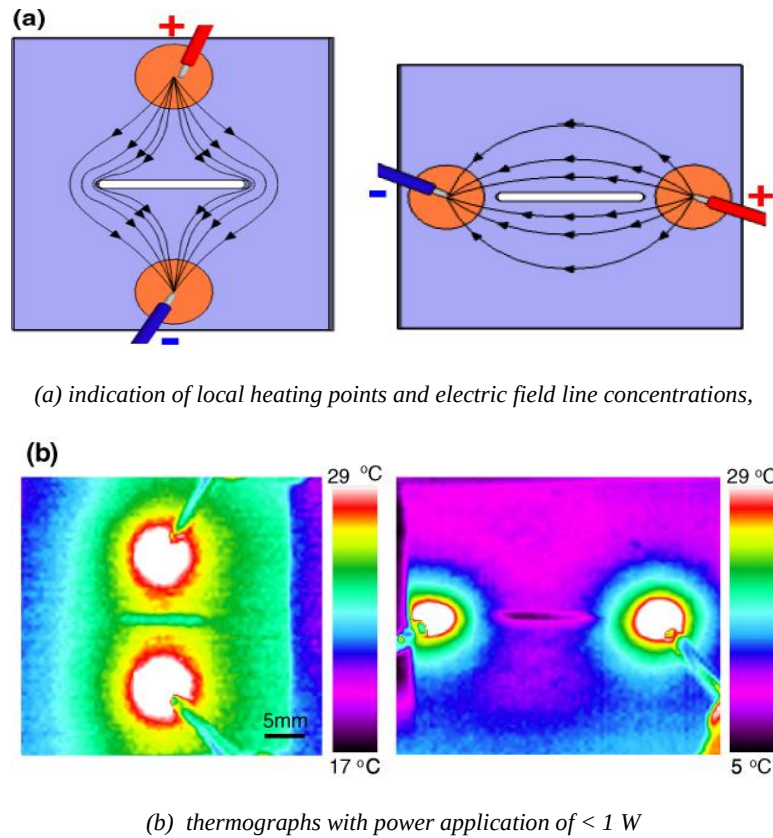
Figure 1-6: Resistive heating of a through-crack in a nanocomposite [2].
