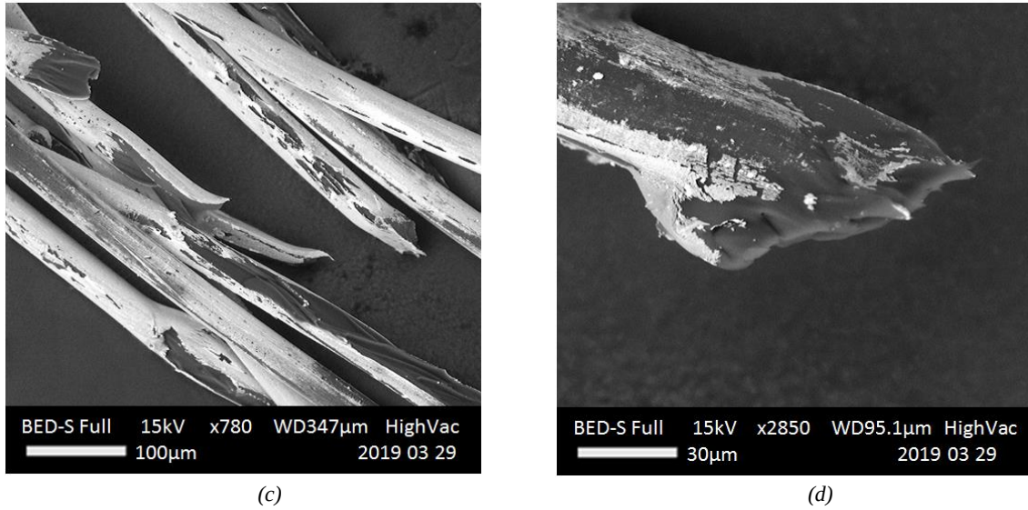
Figure 2-9: SEM characterization of the fractured specimen. (a)-(c) show fractured fibers in each specimen with similar morphologies. (d) shows a single fractured filament of the coated yarn at 30 \mu\text{m} zoom presenting both ductile fracture and pull-out of the coating during large deformation.
