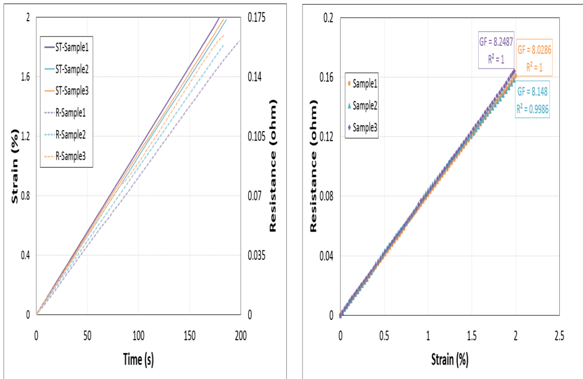
(a) Strain and resistance change
