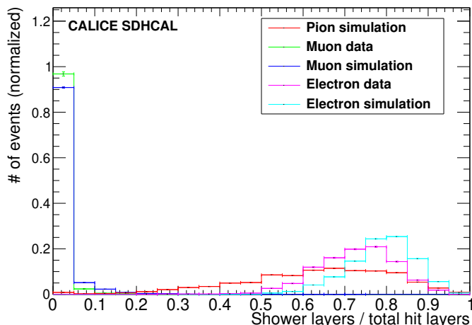
Figure 5.4: Distribution of ratio of the number of layers in which RMS of the hits' position in the x - y plane exceeds 5 cm over the total number of fired layers ( N_{\text{interactingLayers}}/N_{\text{Layers}} ).
