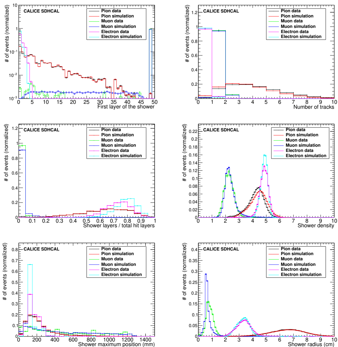
Figure 5.15: Distributions of six input variables of electron, muon and pion samples. Pion distributions are obtained from pion data samples after applying the data-based training BDT selections.
