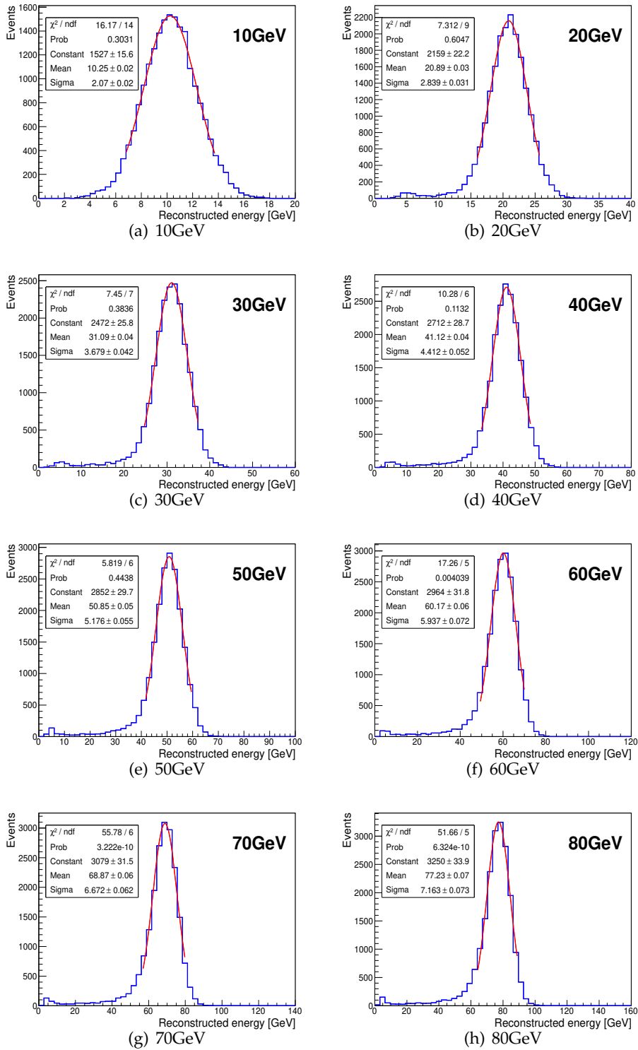
Figure 6.2: Pion energy reconstruction using classical method with energy points 10, 20, 30, 40, 50, 60, 70, 80 GeV samples. The distributions are fitted with a Gaussian function in a \pm 1.65\sigma (RMS > 90%, it means the smallest region include the 90% events) range around the mean value. The mean value and standard deviation of the Gaussian function are treated as the reconstructed energy and its resolution.
