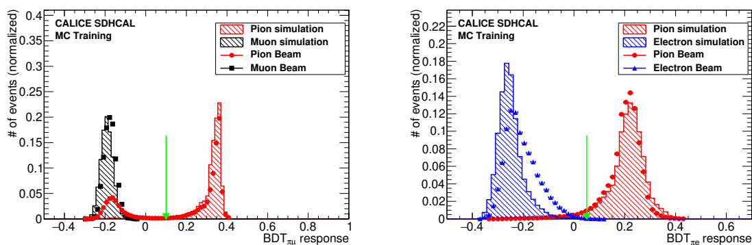
Figure 5.11: The BDT output after using the BDT_{\pi\mu} on the data pion sample (left) and the BDT output after using the BDT_{\pi e} on the same data pion sample after classified by BDT_{\pi\mu} (right). A green arrow is shown on both to indicate the BDT cut applied to clean the pion samples.
