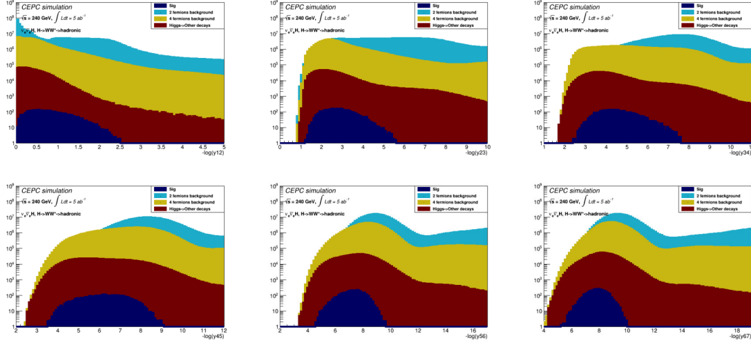
Figure 7.18: The distribution of parameters of jet reconstruction for signal and backgrounds. The number of events for \sqrt{s} = 240 \text{ GeV} and integrated luminosity 5 \text{ ab}^{-1} .
