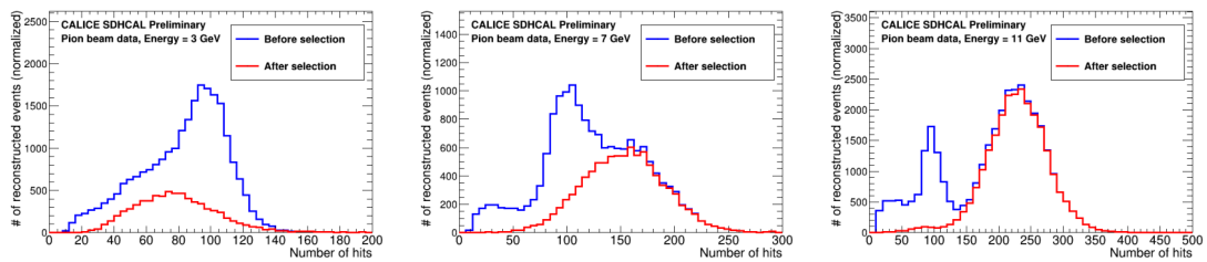
Figure 5.36: The number of hits for 3, 7 and 11 GeV pion beam runs before (blue) and after (red) selection.
