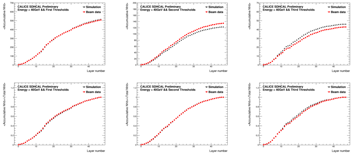
Figure 4.59: The upper three plots show the comparison of number of hits belonging to First(left),Second(middle),Third(right) thresholds as a function of the layer number when intergating over all layers between simulation and data for the 40GeV. The three plots below show the same plots as the upper but using the total number of hits normalized to 1.
