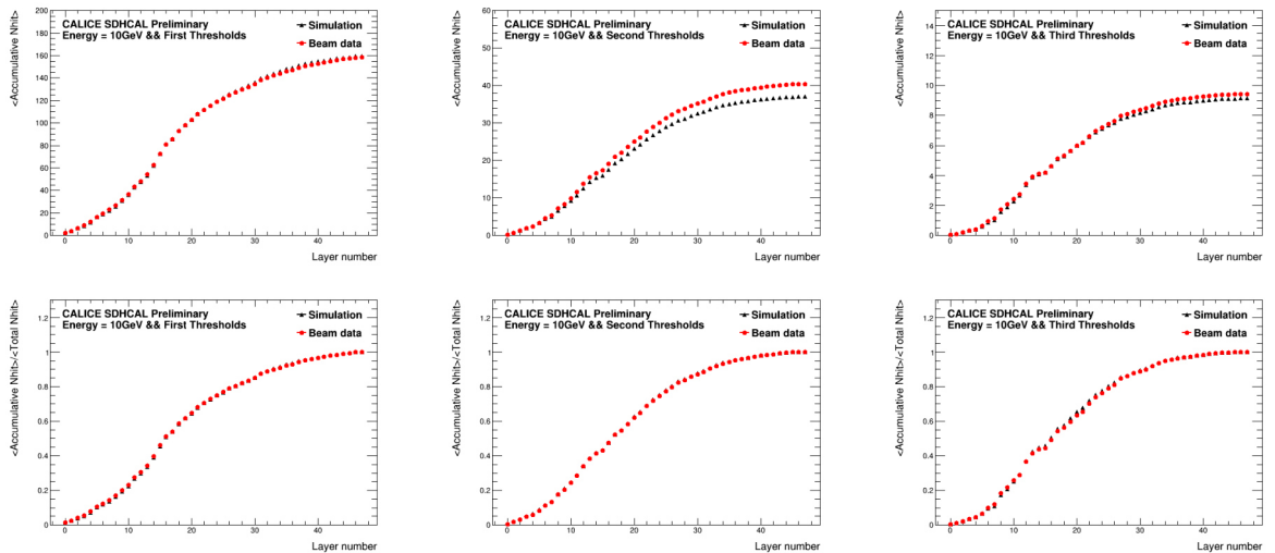
Figure 4.58: The upper three plots show the comparison of accumulated number of hits of first(left), second(middle), third(right) thresholds as a function of the layer number when intergating over all layers between simulation and data for the 10GeV. The three plots below show the same plots as the upper but using the total number of hits normlized to 1.
