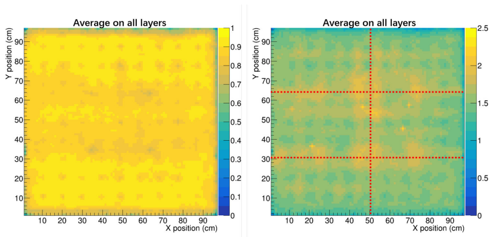
Figure 4.29: Left: the efficiency map \epsilon(x, y) . Right: the multiplicity map \mu(x, y) . Both efficiency and multiplicity maps are averaged on 35 layers. The red dashed lines are related to the borders of six ASU PCBs. The results are obtained from 2018 beam test.
