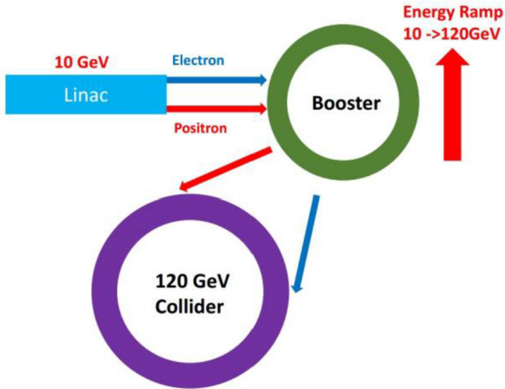
Figure 2.6: The layout of the CEPC injection chain [21].
