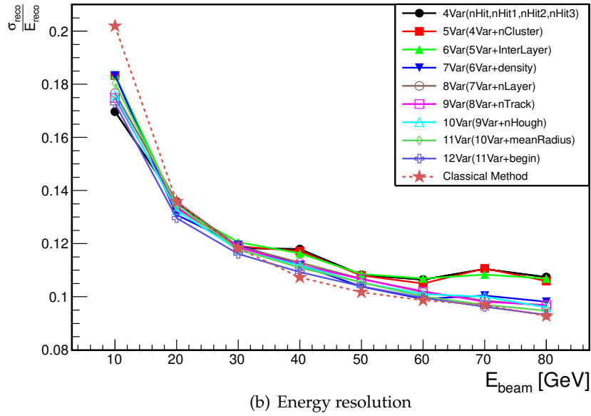
Figure 6.12: The energy deviation from linearity ( \Delta E/E_{beam} ) and resolution ( \sigma/E_{reco} ) of the BDTG with different sets of input variables (from 4 to 12 variables). The colors and markers of the two line charts are the same as the MLP's. The results of classical method are also included in the plot for comparison.
