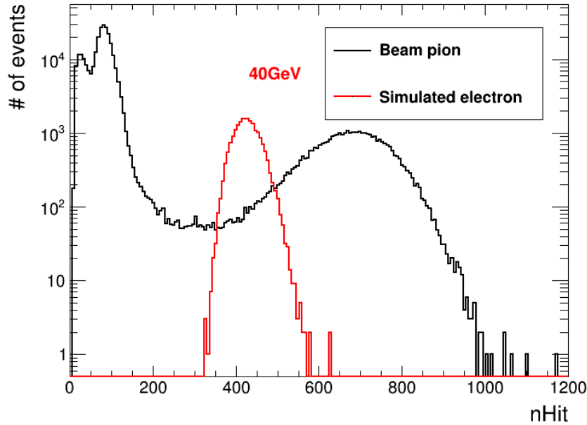
Figure 4.40: The n\text{Hit} distribution of 40 GeV pion beams (black) and simulated electron events (red). It is clear that electron contamination can be hidden by the huge number of pions due to the overlaps of the distributions of them
