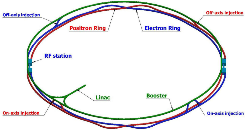
Figure 2.5: The layout of CEPC [21].
