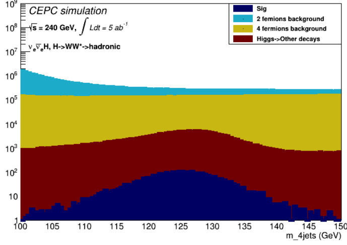
Figure 7.14: The distribution of invariant mass of four jets for signal and backgrounds. The number of events for \sqrt{s} = 240 \text{ GeV} and intergrated luminorsity 5 \text{ ab}^{-1} .
