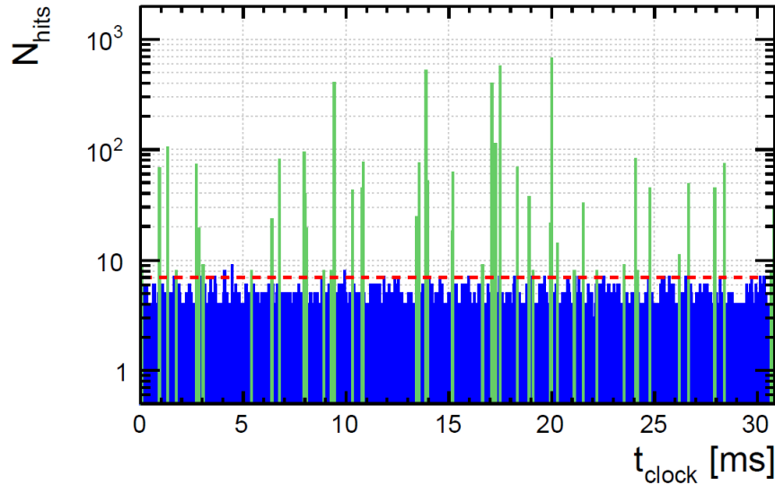
Figure 4.13: The hits - time histograms with time slot 200 ns. The green lines represent the physics event candidates and the blue is from intrinsic noise. The K_{\text{hit}} is presented by the red dashed line. This figure is cited from Ref. [46].
