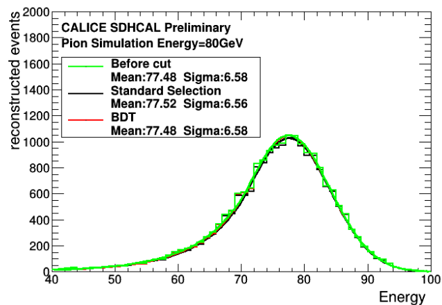
Figure 5.21: The comparison of reconstructed energy between BDT and standard methods using simulation samples for 80 GeV. The distributions are fitted by Crystal Ball functions.
