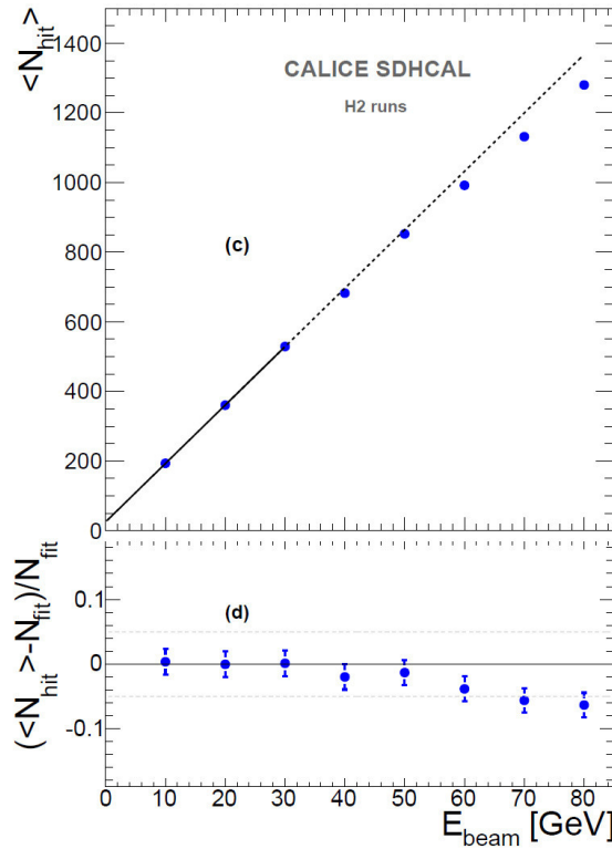
Figure 4.49: The mean of total number of hits as a function of beam energy. The dashed line is a function \langle N_{\text{hit}} \rangle = k * E_{\text{beam}} . The relative deviation \frac{\Delta N_{\text{hit}}}{N_{\text{hit}}} as a function of beam energy is also shown. Right: the mean of number of hits associated with first (green square), second (blue triangle) and third red cross thresholds as a function of beam energy [46].
