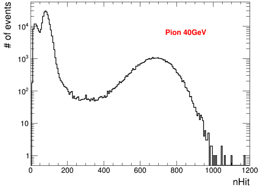
Figure 4.39: The n\text{Hit} distribution of 40 GeV pion beams taken at 2015. The two peaks at the top left are respectively contributed by the cosmic muons and muons produced by beam pion decaying. the relative wider peak at right is contributed by the hadronic showers.
