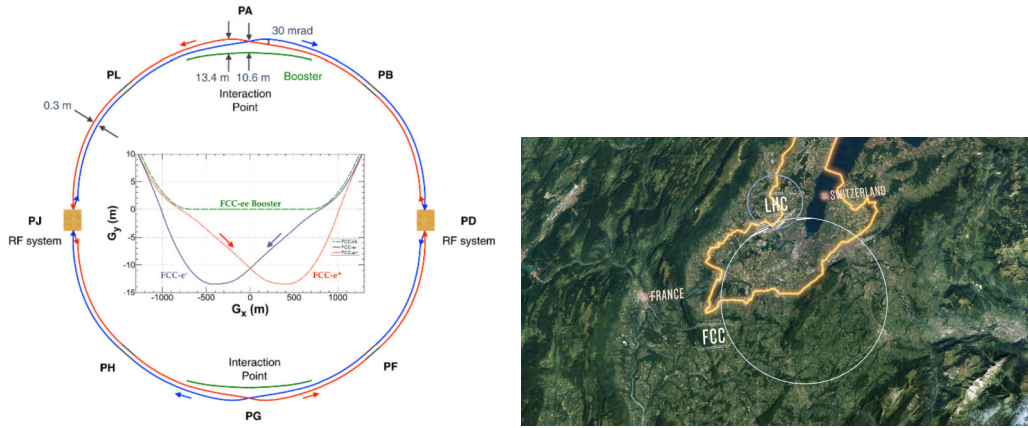
Figure 2.21: Left: The layout of FCC-ee accelerator complex with two IPs. Right: the future location of FCC in the map. The two figures are cited from [39].
