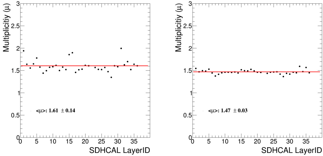
Figure 4.30: Left: the average multiplicities of 35 GRPC layers of SDHCAL prototype before homogenization process. Right: the average multiplicities of 35 GRPC layers after homogenization process. The results are obtained from 2018 beam test.
