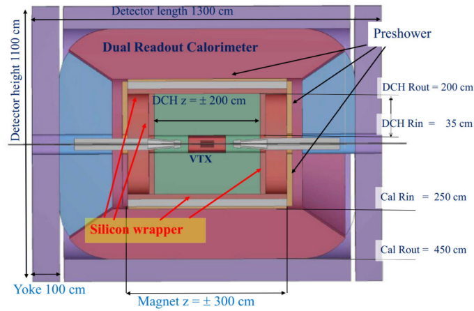
Figure 2.18: The layout of IDEA concept.
