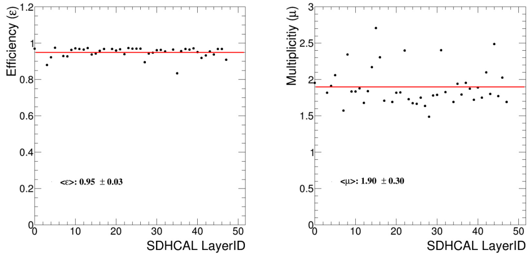
Figure 4.26: Left: the efficiencies of 43 GRPC layers (five layers are not available in the test beam period in 2017) of SDHCAL prototype. Right: the multiplicities of 43 GRPC layers of SDHCAL prototype. The all GRPC layers work at 6.7 kV.
