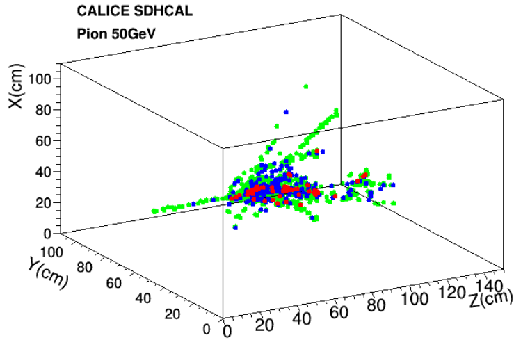
Figure 4.36: The event displays of a 50 GeV pion. Hits pass the first threshold are depicted in green. Hits that pass the second in blue while the those that pass the third threshold are in red.
