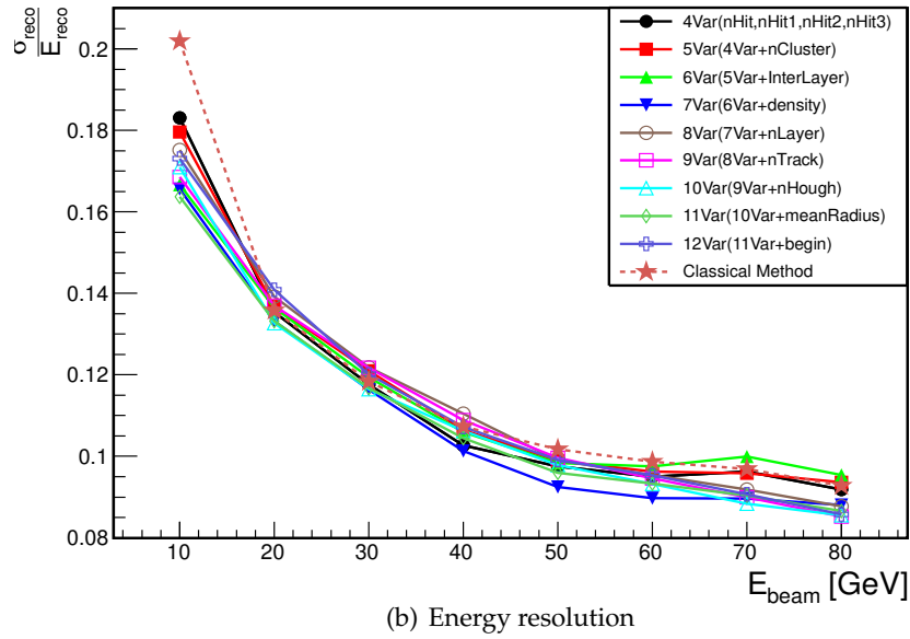
Figure 6.9: The top plot shows the energy deviation from linearity ( \Delta E/E_{beam} ) and bottom one shows the energy resolution ( \sigma/E_{reco} ) results (from 4 to 12 variables) with MLP method. Different colors and markers denote for different sets of input variables. The variables are added one by one following the order of the strength of their correlation with the beam energy.
