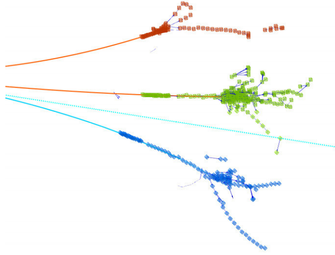
Figure 7.6: The illustration of clustering reconstruction of Arbor PFA in the CEPC detector. The 3-prong decay of \tau -lepton from Z \rightarrow \tau^+ \tau^- . Three reconstructed branches of calorimeter clusters represent a 5.7 GeV \pi^+ (red), a 27.4 GeV \pi^+ (green) and a 10.3 GeV \pi^- (blue). The Monte Carlo truth information of two \pi^{+} 's (red line), a \pi^- (cyan line) and a \bar{\nu}_\tau (cyan dashed) [20].
