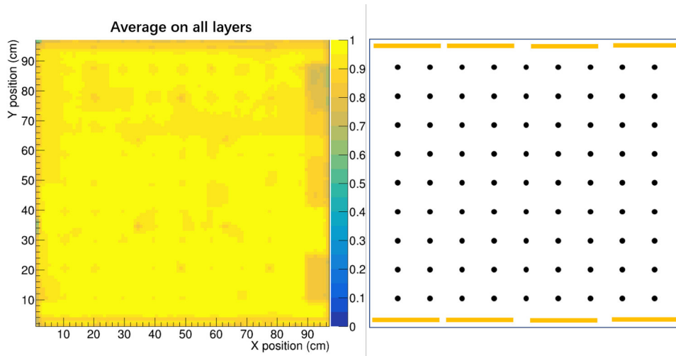
Figure 4.23: The efficiency map \epsilon(x, y) average on all layers shown in the left figure. The impact on efficiency due to spacers, gas channeling pipes is shown in the right figure. The results are obtained from 2015 beam test.
