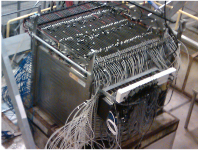
Figure 2.15: The SDHCAL technological prototype exposed in the test beam.
