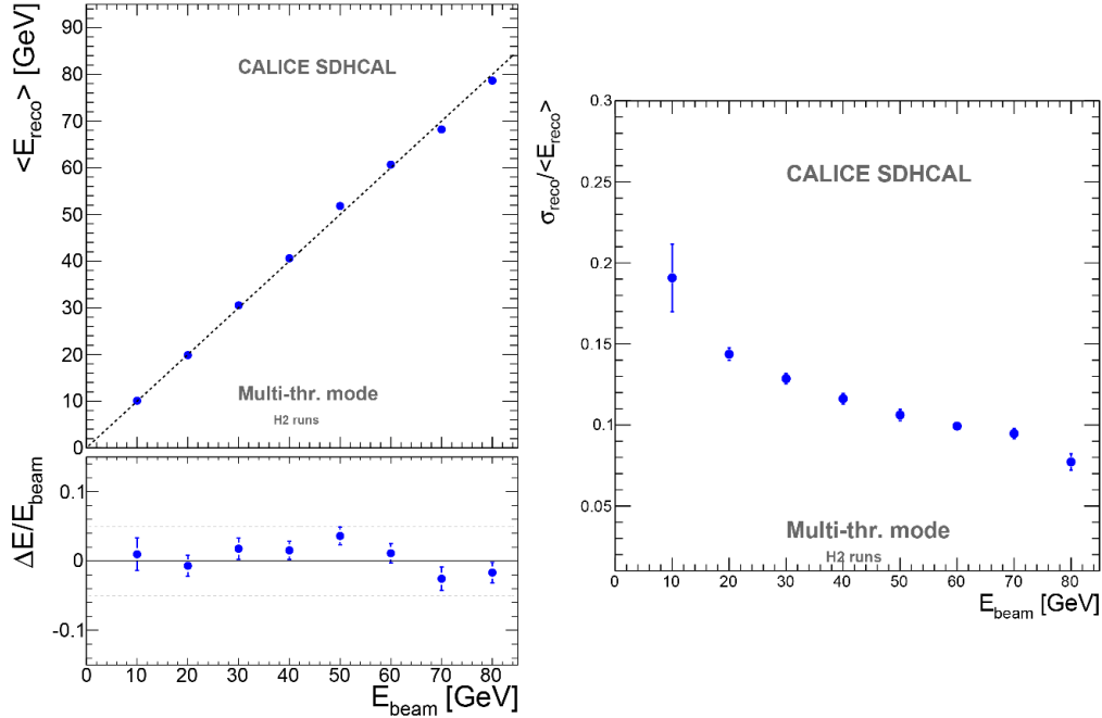
Figure 4.55: Left: The mean of reconstructed energy and the relative deviation \frac{\Delta E}{E} as a function of beam energy in multi-threshold mode. Right: the energy resolution as a function of beam energy in multi-threshold mode [46].
