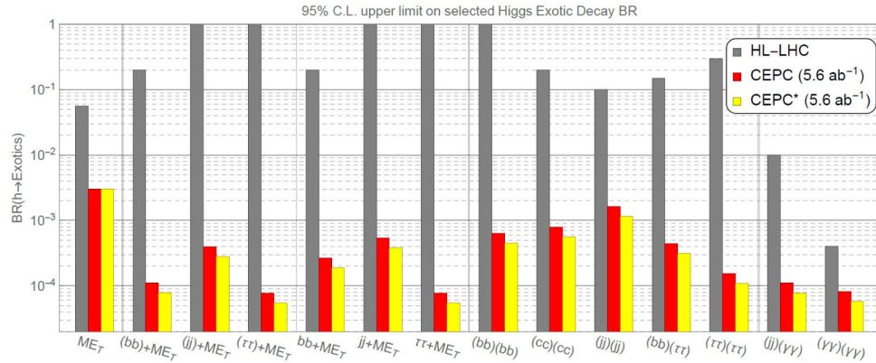
Figure 2.3: The 95%CL upper limit on selected Higgs exotic decay branching fractions at HL-LHC and CEPC, based on Ref. [24]. The red bars is from the results using only leptonic decays of the spectator Z-boson. The yellow bars include extrapolation with the inclusion of the hadronic decays of the spectator Z-boson. This figure cited from Ref. [20].
