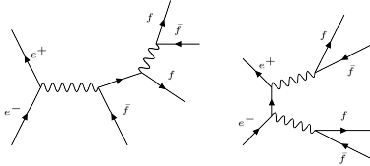
Figure 7.10: The Feynman diagrams for main process for four-fermions background.
