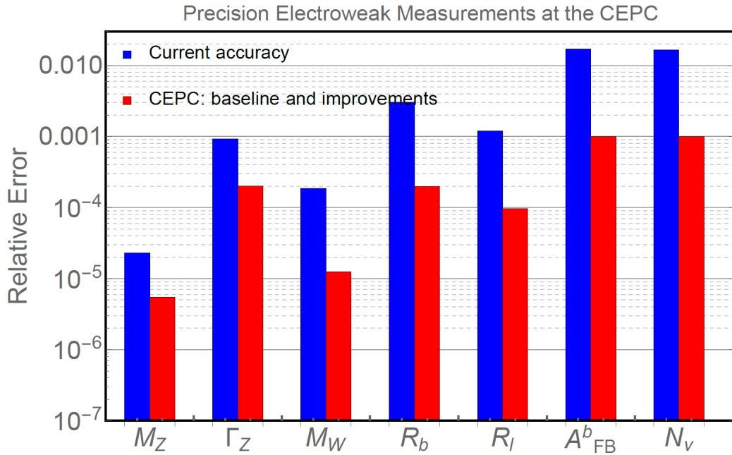
Figure 2.2: The projection for the precision of the electroweak measurements of CEPC in Z-factory mode [20].
