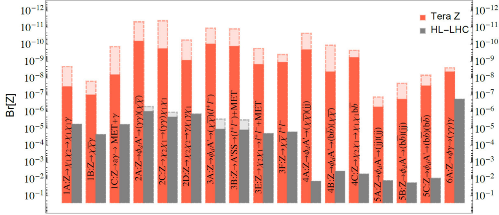
Figure 2.4: The sensitivity of Z branching ratio for different exotic Z decay channels at CEPC ( 10^{12} Z ), and the HL-LHC at 13 TeV with L = 3ab^{-1} , based on Ref. [25]. This figure cited from Ref. [20].
