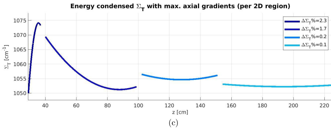
Figure 7.27: For each polynomial layer, the figures show the maximum axial gradients of the total macroscopic cross section among all 2D regions and energy groups (a), integrated over the radial plane, among all groups (b) and energy-condensed, among all 2D regions (c). All plots refer to 60 GWd/t .
