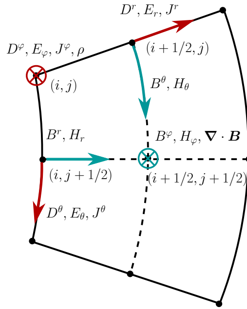
FIGURE 10.3: Yee grid in spherical coordinates. The red arrows denote the components of the electric fields, the blue ones denote the magnetic fields. The positions on the mesh are labelled by the indices i in the radial direction and j in the orthoradial direction.
