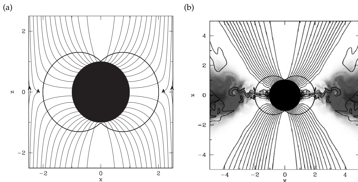
FIGURE 3.2: (a) Steady-state force-free simulation of a black hole immersed in a vertical magnetic field. The magnetic flux is pulled onto the event horizon. (b) Quasi-steady state of a GRMHD simulation of an accretion flow around a Kerr black hole with a = 0.999 . The solid lines show poloidal magnetic field lines. Figures taken from Komissarov & McKinney (2007) .
