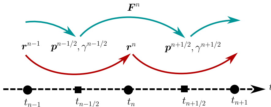
FIGURE 9.2: Illustrative diagram of the leapfrog scheme for the particles. The positions are defined at integer time steps, whereas the velocities are defined at half-integer time steps.
