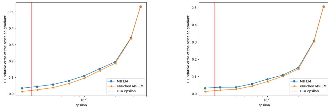
Figure 3.19: H_\varepsilon^1 relative error in log scale, for H = 1/32 , h = 1/768 , f = f_1 (bending case), A^\varepsilon = A_{\text{per},0}(\cdot/\varepsilon, \cdot) (left) and A^\varepsilon = A_{\text{per},1}(\cdot/\varepsilon, \cdot) (right)
