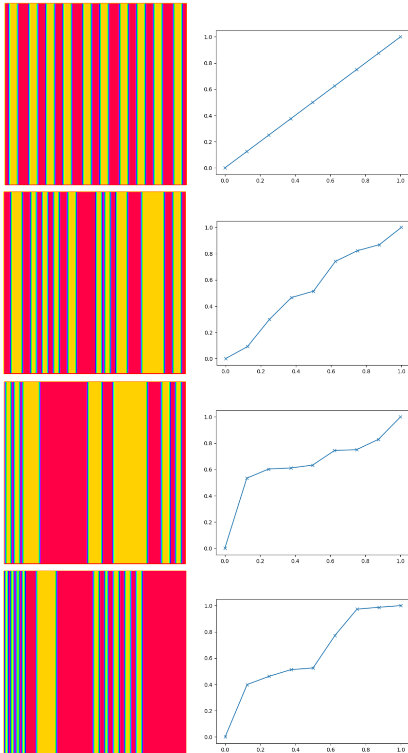
Figure 4.1: Plots of E^{\psi,\varepsilon} and \psi for different functions \psi in \mathcal{U}^{H_{\text{diff}}} .
