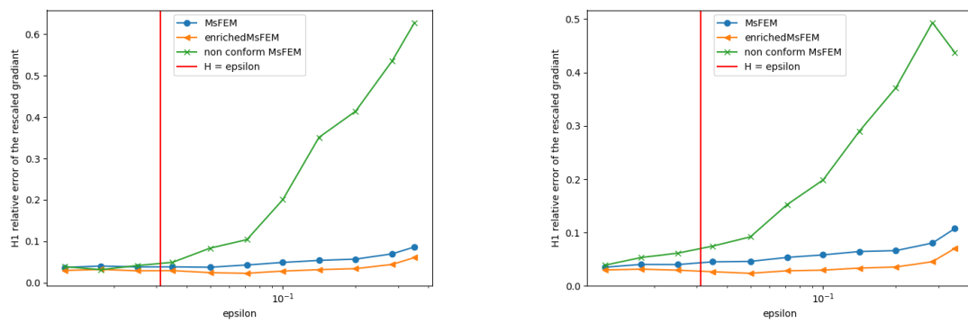
Figure 3.20: H_\varepsilon^1 relative error in log scale, for H = 1/32 , h = 1/768 , f = f_0 (membrane case), A^\varepsilon = A_{\text{per},2}(\cdot/\varepsilon, \cdot) (left) and A^\varepsilon = A_2(\cdot/\varepsilon, \cdot) (right)
