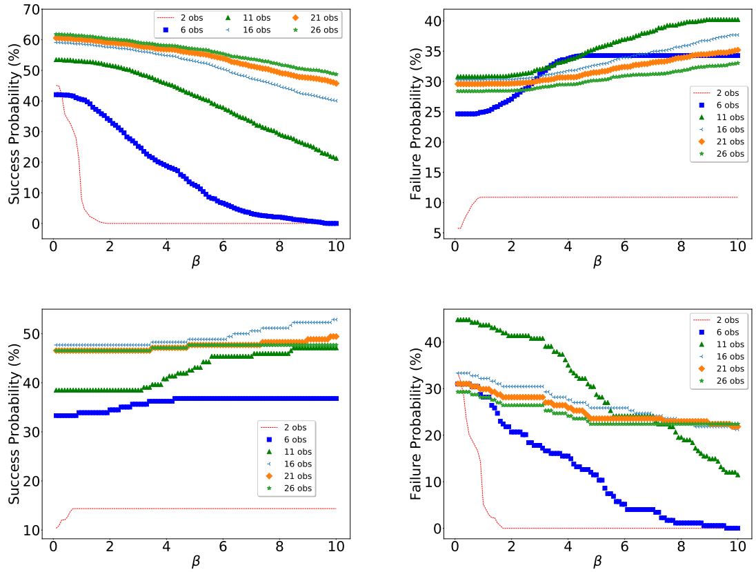
Fig. 4.6 The success (left) and failure (right) probabilities versus \beta . The preferred event is reported after 2, 6, 11, 16, 21 and 26 observations. The top (bottom) panels correspond to “SN” (respectively “Others”) type objects.
