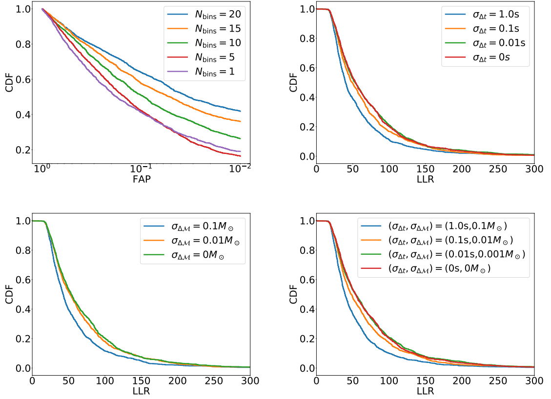
Fig. 3.7 Top left: CDF versus FAP, for the case of signals injected and recovered with the same binary parameters. Top right: CDF versus LLR for injected signals with \sigma_{\Delta \mathcal{M}} = 0 and different values of \sigma_{\Delta t} . Bottom left: CDF versus LLR for injected signals with \sigma_{\Delta t} = 0 and different values of \sigma_{\Delta \mathcal{M}} . Bottom right: CDF versus LLR for different values of (\sigma_{\Delta t}, \sigma_{\Delta \mathcal{M}}) . For all the panels, except the top left, the setting N_{\text{bins}} = 10 is used.
