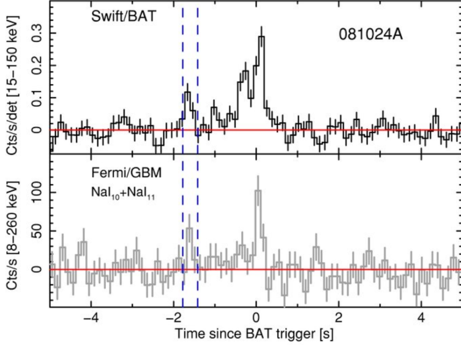
Fig. 3.1 Swift /BAT and Fermi-GBM lightcurves of GRB 081024A, containing two statistical significant bursts of photons. The picture is taken from Troja et al. [2010].
