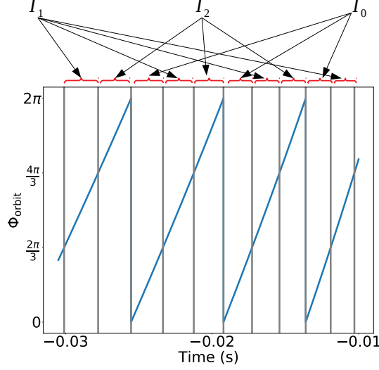
Fig. 3.3 The positions of I_0 , I_1 and I_2 , for N_{\text{bins}} = 3 . In blue, orbital phase \Phi_{\text{orbit}} versus time. The origin of the x axis corresponds to the merger time.
