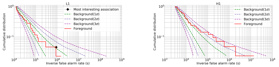
Fig. 2.11 On left (right), the cumulative density function of the inverse false alarm rate for the background and the foreground associations when the LIGO-Livingston (respectively LIGO-Hanford) GW triggers are considered. For the background associations, the 1\sigma , 2\sigma and 3\sigma uncertainties are provided too. On the left plot, the diagram coordinates of the most interesting foreground association is equally provided.
