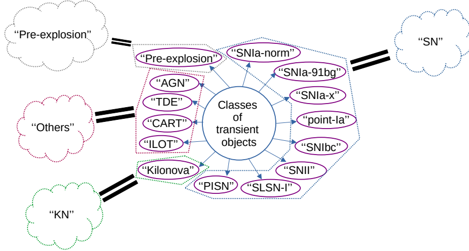
Fig. 4.3 Initial guess of the four main classes, obtained by the collapse of original astorapid classes.
