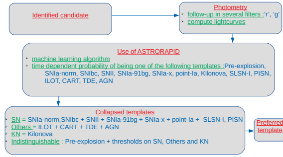
Fig. 4.7 Flowchart showing the different steps of the analysis. The photometric multi filter input data is initially analyzed by astorapid which offers, after each new observation, a probability distribution over fourteen templates. The astorapid output is manipulated as described in this section in order to report, at each new observation, a preferred template from {“SN”, “Others”, “KN”, “Indistinguishable”}.
