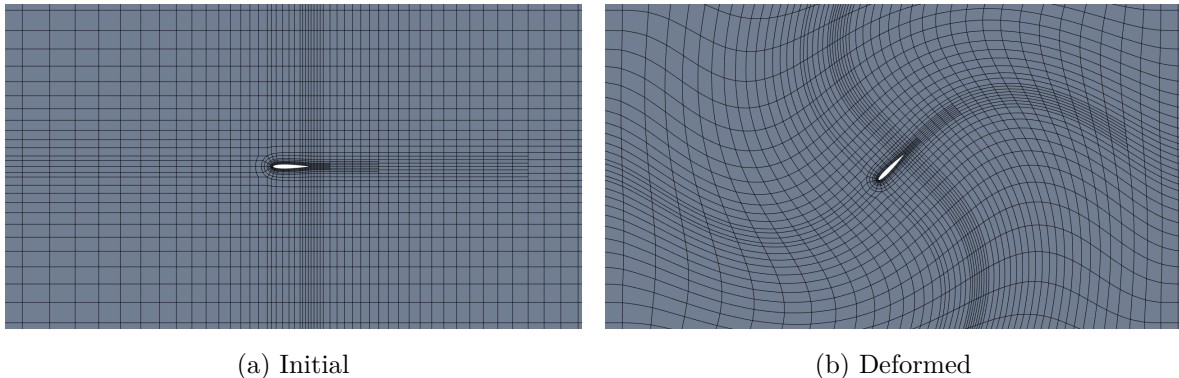
Figure 2.1: Mesh movement example
