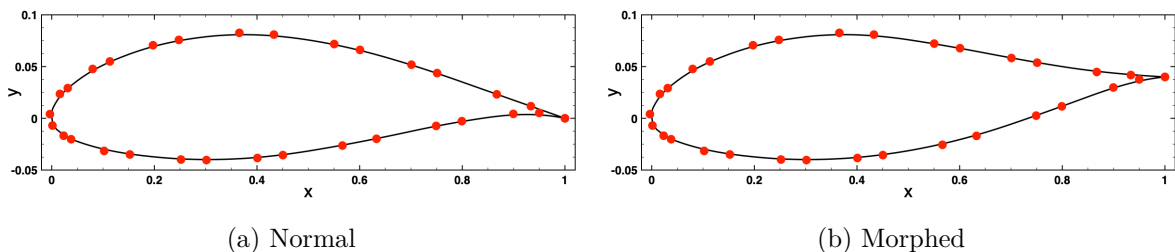
Figure 4.1: B-Spline representation of the NACA 63 1 – 412 airfoil
