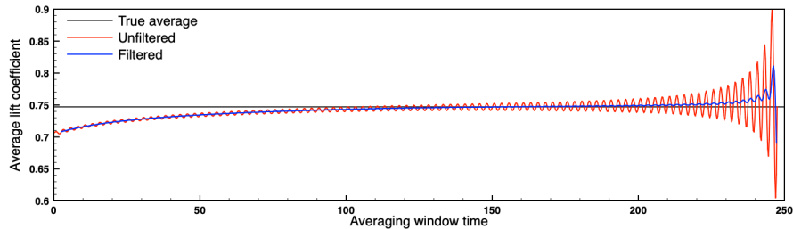
(b) Average lift coefficient
