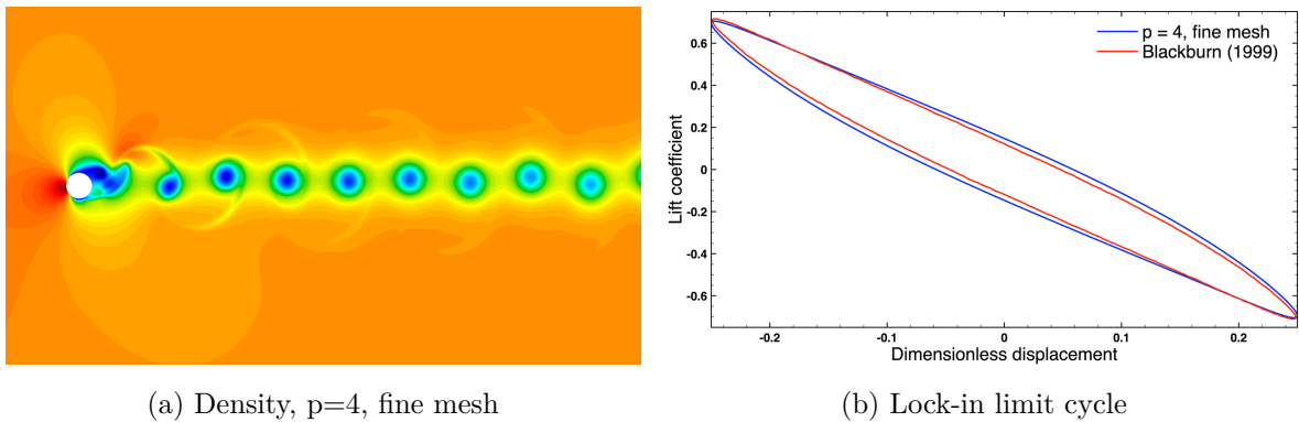
Figure 2.9: Numerical solution of the oscillating cylinder test case
