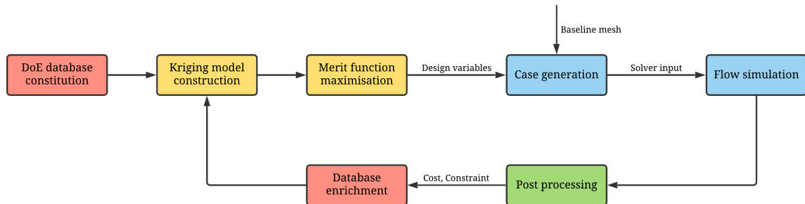
Figure 4.12: Optimisation workflow
