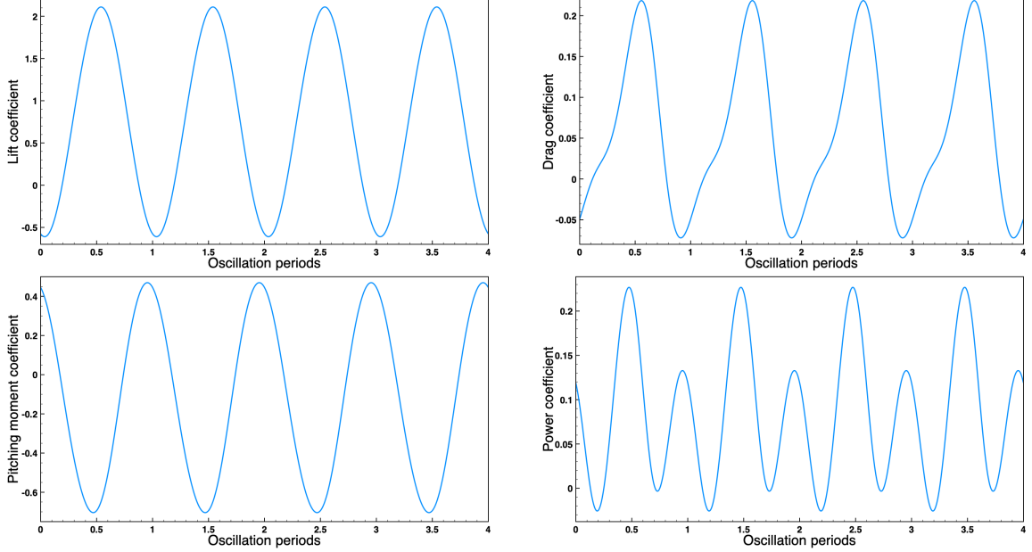
Figure 4.8: Morphing airfoil, evolution of the aerodynamic coefficients
