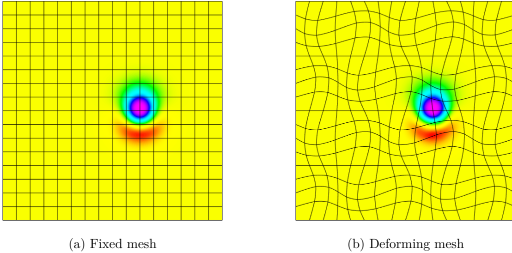
Figure 2.6: Isentropic vortex, energy, t=1.25 , p=3
