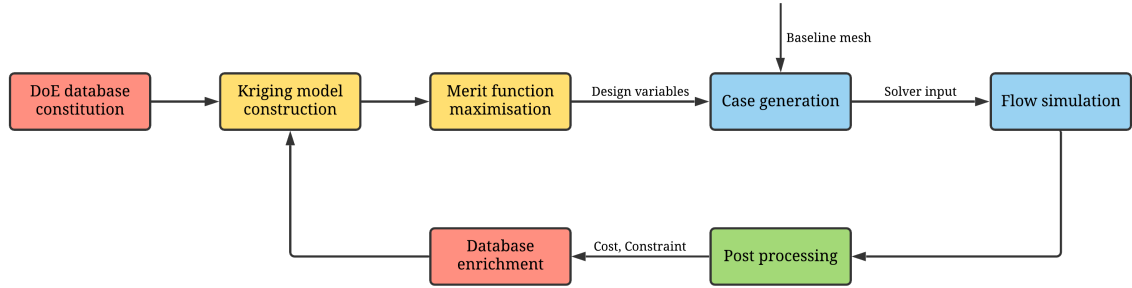
Figure 4.12: Optimisation workflow
