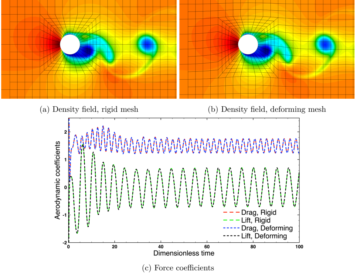
Figure 2.10: Comparison of movement laws, p=5 , intermediate mesh
