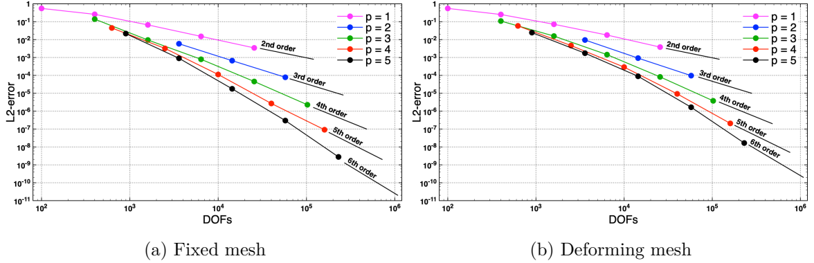
Figure 2.7: Convergence analysis, Euler equations, L^2 -error of total energy
