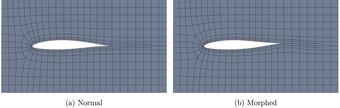
Figure 4.4: Morphing of the refined mesh
