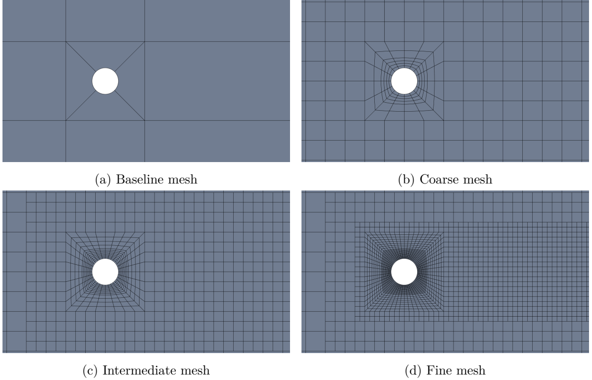
Figure 1.8: Different refinement levels for the cylinder simulation
