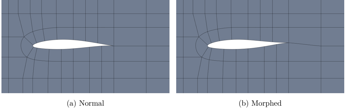
Figure 4.3: Morphing of the baseline mesh
