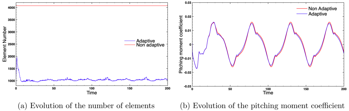
Figure 2.22: Transonic pitching NACA airfoil, results comparison
