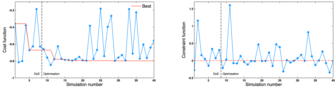
Figure 4.19: Second run, DOE and EGO iterations
