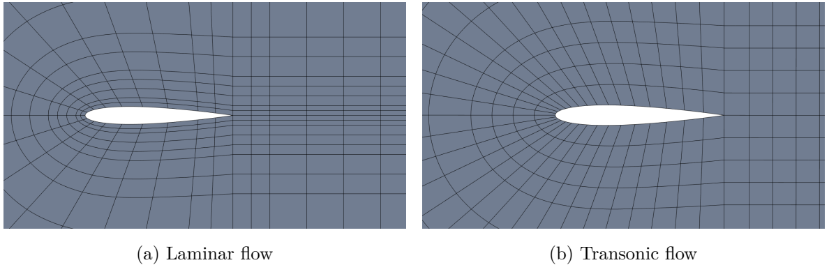
Figure 2.18: Baseline meshes for adaptive pitching airfoil simulation
