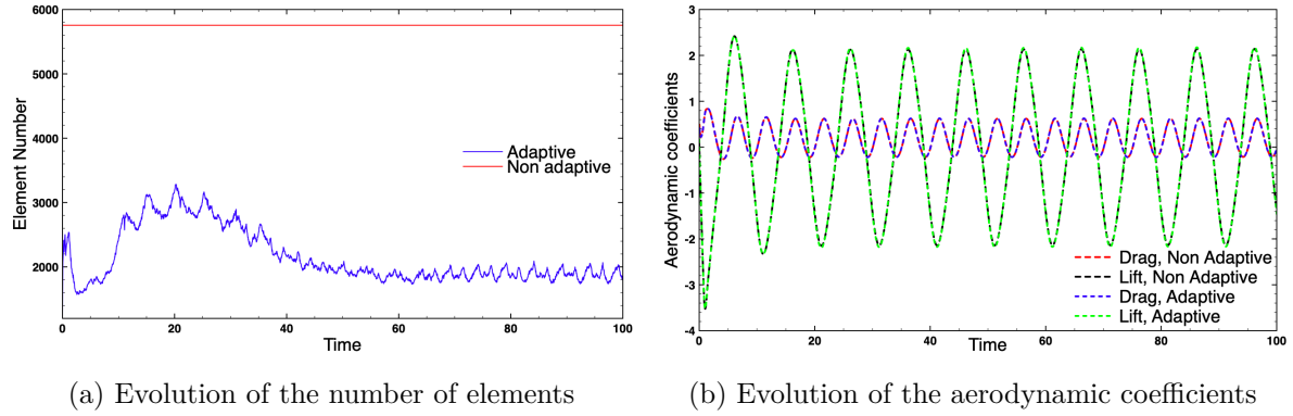
Figure 2.20: Laminar pitching NACA airfoil, results comparison
