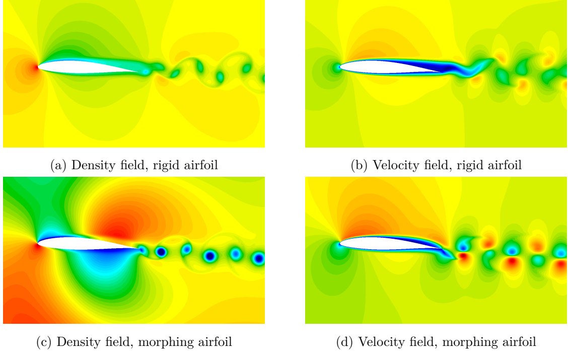
Figure 4.9: Comparison of rigid and morphing airfoil flows, fine grid
