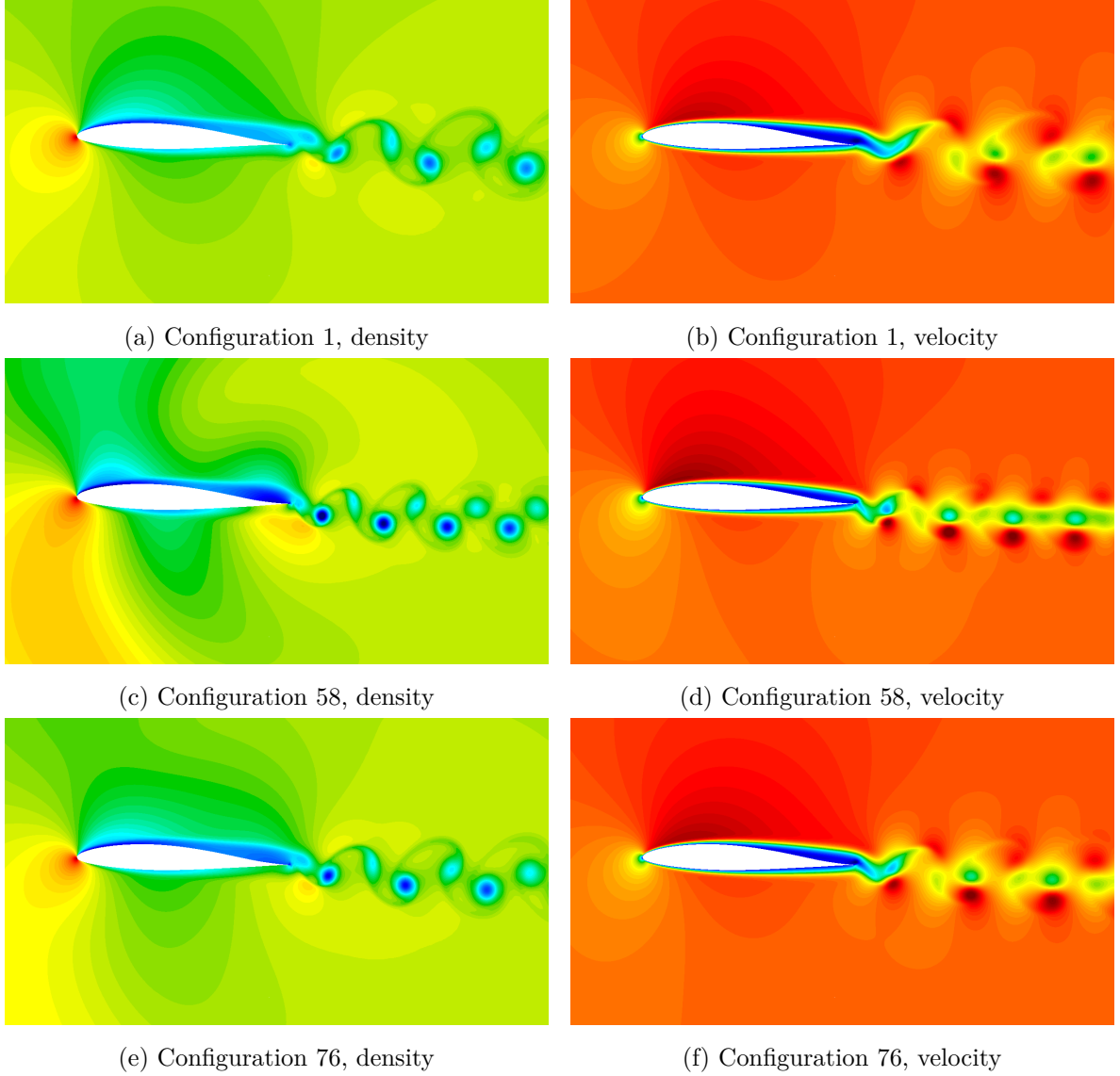
Figure 4.28: Multi-objective optimisation, solution fields
