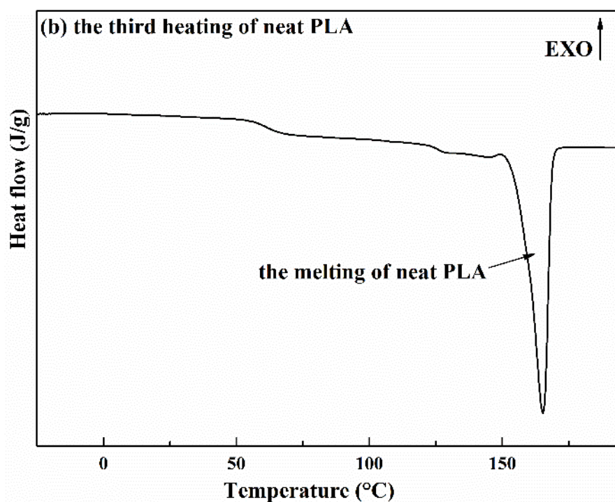
Figure 2-6 The DSC curves of neat PLA electro sprayed microspheres (a) the second heating process and (b) the third heating process.
