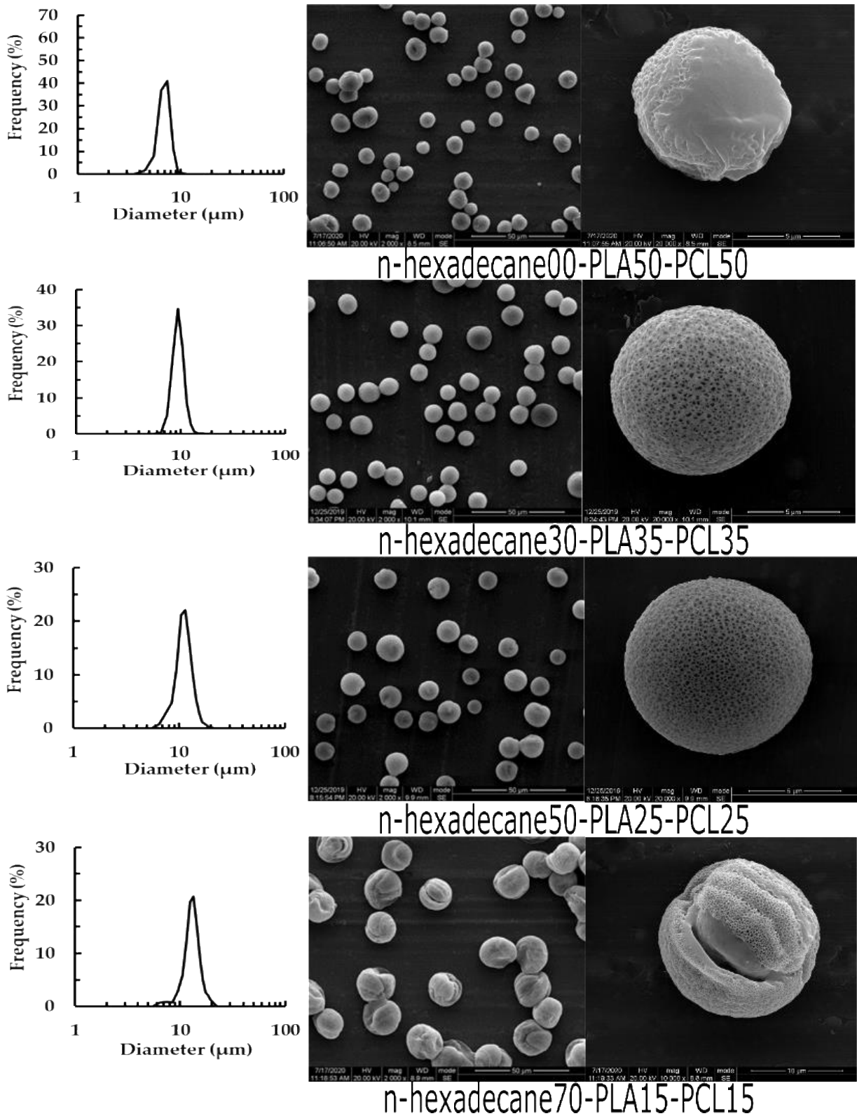
Figure 7-1 The SEM images and size distribution of PLA/PCL microparticles and a series of n-hexadecane/PLA/PCL electrospayed mPCMs with different n-hexadecane additions.
