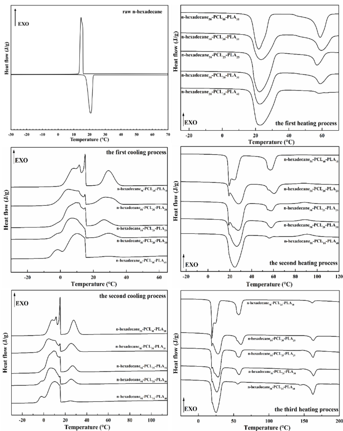
Figure 7-4 The DSC curves of raw n-hexadecane and a series of n-hexadecane/PLA/PCL microcapsules with different weight fractions between PLA component and PCL component.
