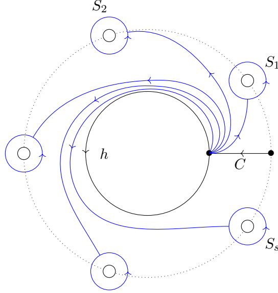
Figure 3.4: The paths for expressing the monodromies of a Stokes local system.
