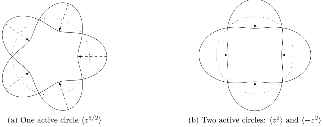
Figure 3.1: Stokes diagrams for two examples of irregular classes. The diagram represents the growth rate of the exponential factors as a function of the direction around the singularity. The dotted circle separates when the exponential factor is growing or decreasing. The Stokes arrows are also represented.
