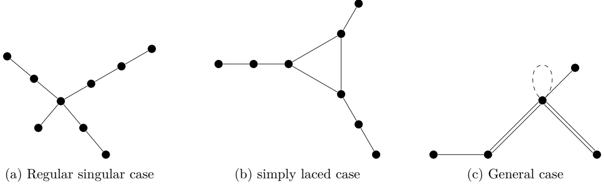
Figure 2.2: Examples of diagrams associated to connections
