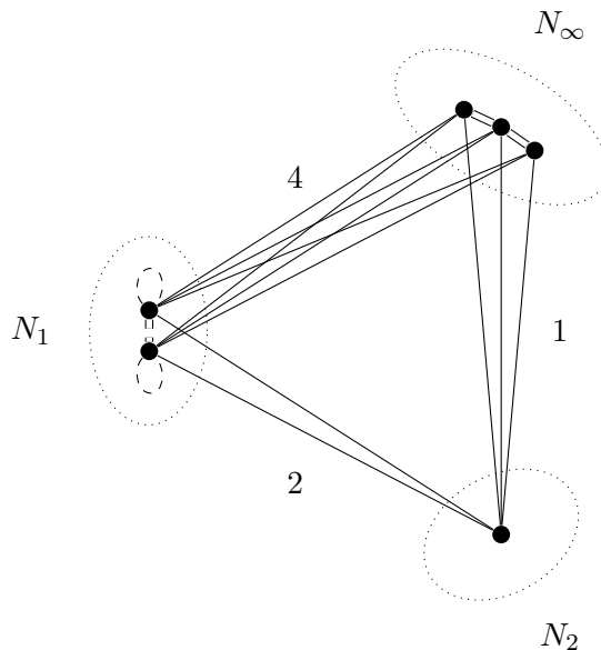
Figure 6.5: An example of core diagram with the partition of the set of nodes N = N_\infty \cup N_1 \cup N_2 . The integers indicate the multiplicities of the edges.
