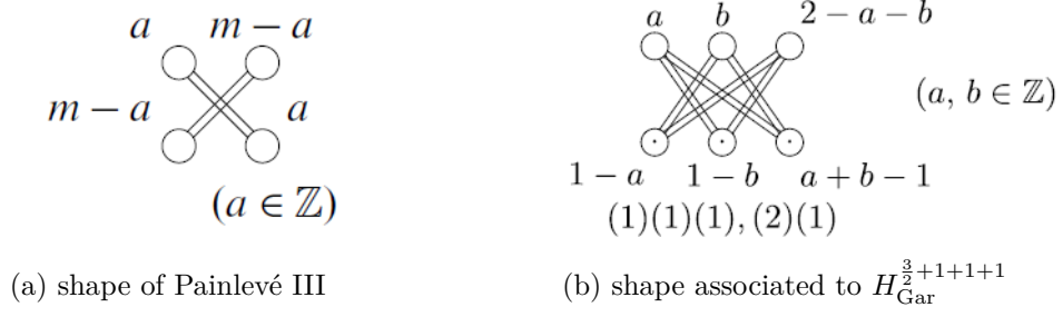
Figure 6.4: Shapes associated to some Painlevé-type equations in [65, 55].
