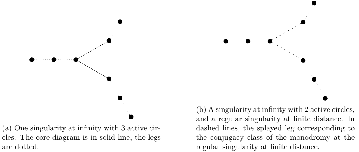
Figure 3.9: Two different readings of the same supernova quiver.
