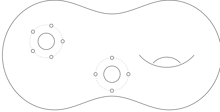
Figure 3.3: Global picture of a Stokes local system: at each singularity there is a halo with tangential punctures.
