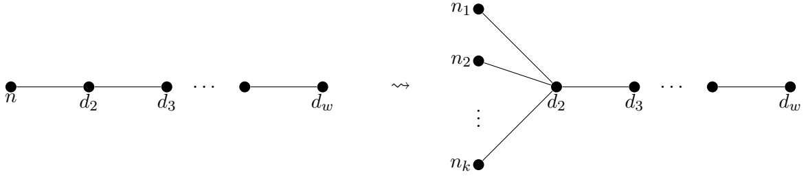
Figure 3.7: Splaying a leg corresponding to the conjugacy class of a regular singularity at finite distance, to glue it to the core diagram with vertices \langle q_1 \rangle, \dots, \langle q_k \rangle .
