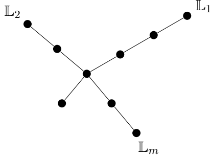
Figure 3.6: Star-shaped quiver associated to a connection with regular singularities.
