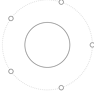
Figure 3.2: Local picture: the halo and the tangential punctures at a singularity.
