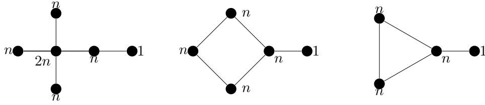
Figure 6.2: Diagrams for higher Painlevé systems hP_{VI}^{(n)} , hP_V^{(n)} , hP_{IV}^{(n)} .
