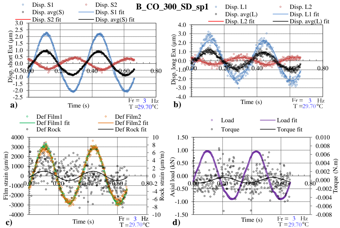
Figure 6-15 Complex modulus tests results of B_CO_300_SD_sp1 at 30^\circ\text{C} and 3\text{Hz} : a) displacement measured by small extensometers, b) displacement measured by long extensometers, c) calculated strains in film and rock phases, d) axial load and torque, all as a function of time
