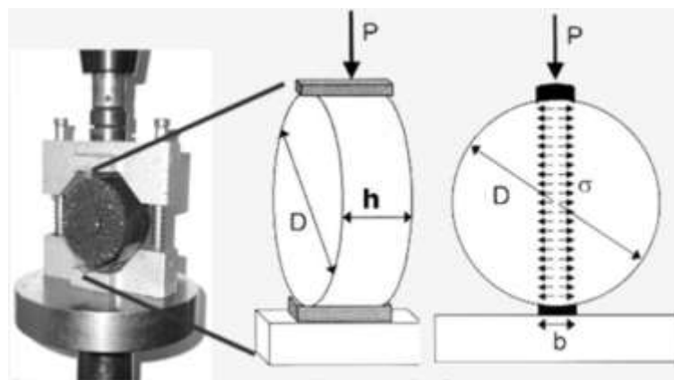
Figure 3-11 Indirect Tensile test set up (Grönniger, Wistuba, and Renken 2010)
