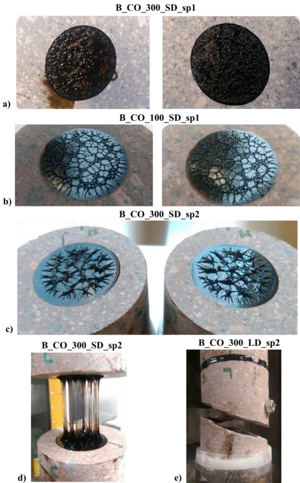
Figure 6-23 Tension failure profile for a) B_CO_300_SD_sp1, b) B_CO_100_SD_sp1, c) B_CO_300_SD_sp2. d) Remnant of bitumen filaments at the end of the tension test on B_CO_300_SD_sp2. e) Tension failure of rock in large-diameter film geometry B_CO_300_LD_sp2
