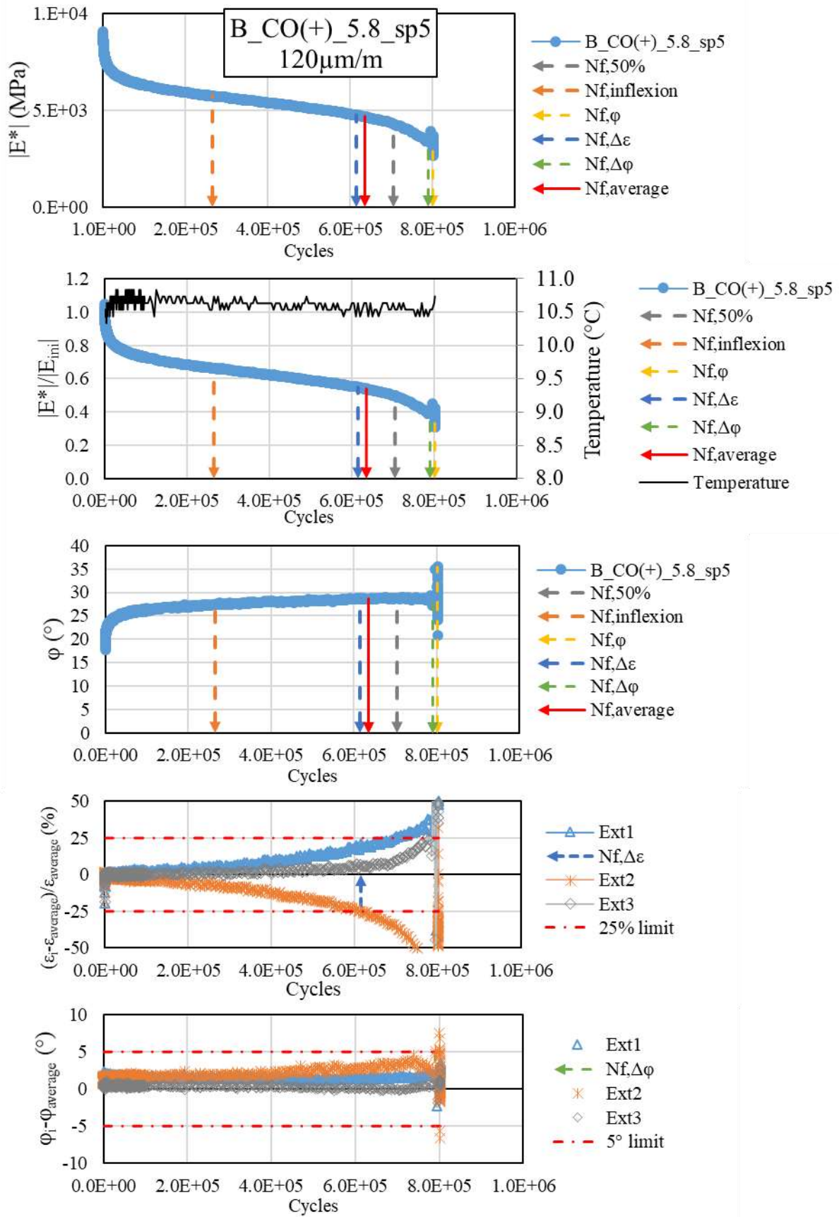
Figure 7-18 fatigue test results of B\_CO(+)\_5.8\_sp5 with TC test at 10^{\circ}C/10Hz , and a strain amplitude of 120\mu m/m
