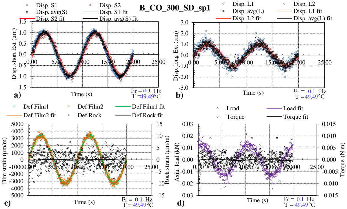
Figure 6-14 Complex modulus tests results of B_CO_300_SD_sp1 at 50^\circ\text{C} and 0.1\text{Hz} : a) displacement measured by small extensometers, b) displacement measured by long extensometers, c) calculated strains in film and rock phases, d) axial load and torque, all as a function of time
