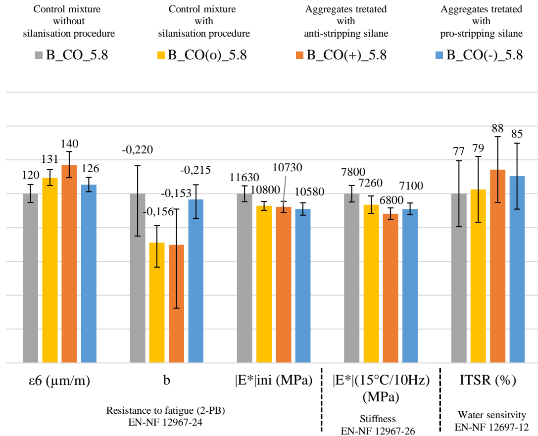
Figure 7-22 Resistance to fatigue with 2-PB apparatus, stiffness and water sensitivity of mixtures with silane-treated aggregates (B_CO(+)_5.8 and B_CO(-)_5.8) and of control mixtures B_CO_5.8 and B_CO_5.8(o). Error bars for the linear regression parameters \epsilon_6 and b represent 95% confidence interval. Error bars for |E^*|_{ini} and |E^*|(15^\circ\text{C}/10\text{Hz}) represent the observed standard deviation. Error bars for the ITSR represent the 95% confidence interval of repeatability (non-consensual value)
