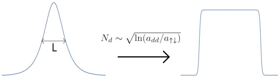
Figure 3.5: Density probability function of the system of dimers before and after the soliton- droplet crossover by increasing the number of dimers N_{\text{d}} .
