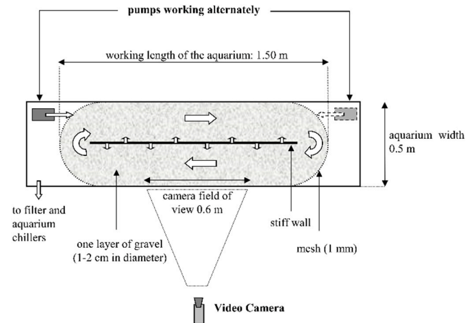
Fig. 2. Diagrammatic top view of the annular flume.
