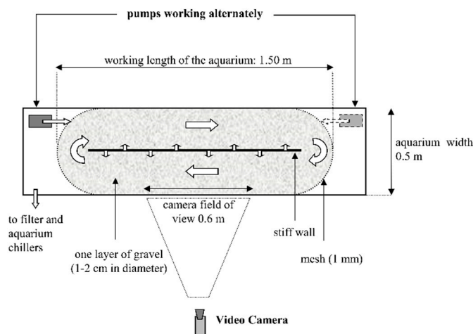
Fig. 2. Diagrammatic top view of the annular flume.
