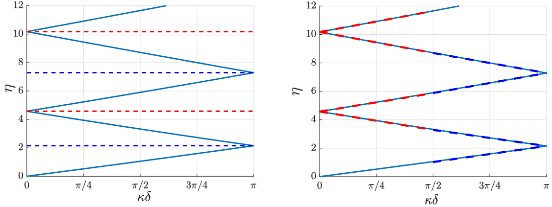
Figure 6.9 – Dispersion diagram for the monolayer case with \mathcal{K} = 2 and \mathcal{M} = 0.5 corresponding to double eigenvalues. (Left) In red (resp. blue) dashed lines are the periodic (resp. antiperiodic) eigenvalues \eta_0 calculated by finding the roots of (6.87). (Right) In red (resp. blue) dashed lines are the periodic (resp. antiperiodic) resulting first-order approximations (6.72).
