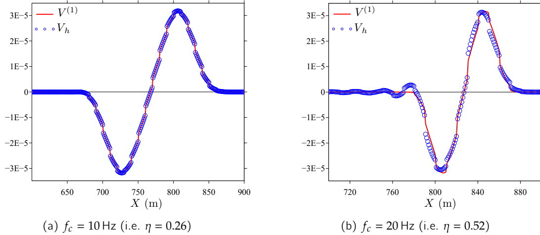
Figure 5.3 – Superposition of the fields V_h and V^{(1)} (in m/s) at t = 0.16 \text{ s} in the case of a homogeneous periodic cell for two different central frequencies.
