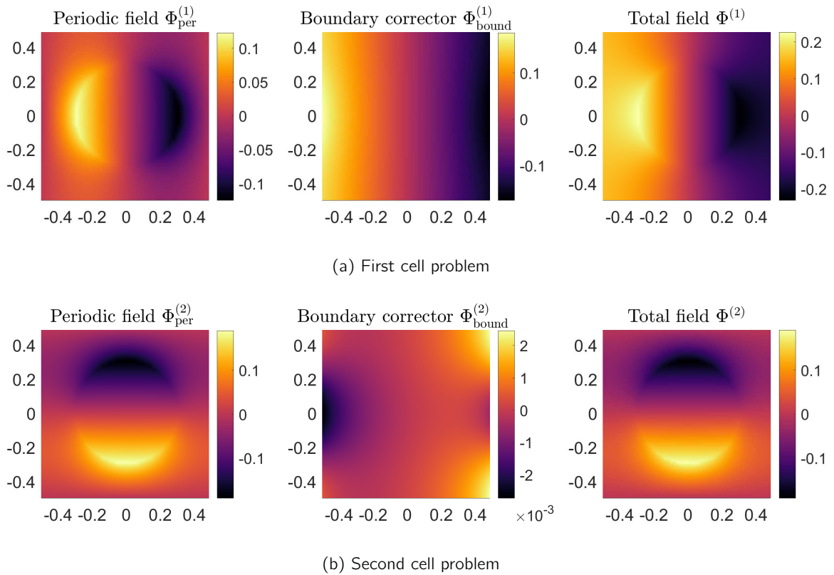
Figure 4.4 – Periodic part, boundary corrector and total fields \boldsymbol{\Phi} .
