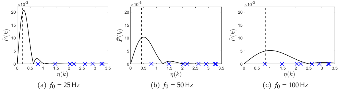
Figure 2.5 – Fourier transform \hat{F} of the source function for the three different values f_0 considered (the associated dimensionless parameters \eta_0 are indicated by the dashed lines). The blue crosses denote the values \eta_r associated with resonances \omega_r , see (1.24), of non-zero mean modes.
