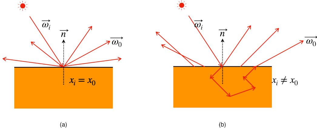
Figure 2.13: Scatttering of light using BRDF (a), and BSSRDF (b).
