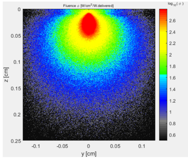
Figure 2.20: Fluence rate map of a three-layered tissue obtained by the MC simulations
