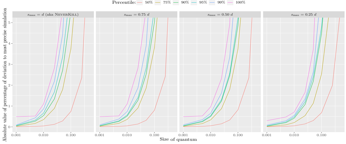
Figure 4.3: Absolute value of percentage of deviation from the performance of the heuristic SMAX, while fixing different values of s_{\max} , predicted for different quantum values, to the performance simulated with 10^7 tasks. For each quantum size and each value of s_{\max} , many different periods, deadlines, and distributions are evaluated whose percentiles (and worst-case) are presented.
