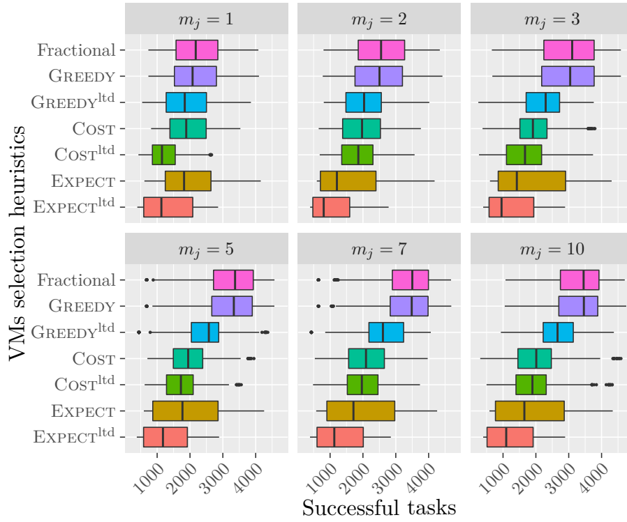
Figure 2.4: Number of successfully executed tasks of different methods to choose VMs when interrupting tasks with heuristic OPT RATIO . Each of the 100 platforms is generated with m_j = 1, 2, 3, 5, 7, 10 , M = 6, 12, 18, 30, 42, 60 , c_j = s_j and is used 10 times with b = 630 and d \approx 13.2 ( K \approx 47.8 ). Execution times follow lognormal distributions with x_{CV} = 3 .
