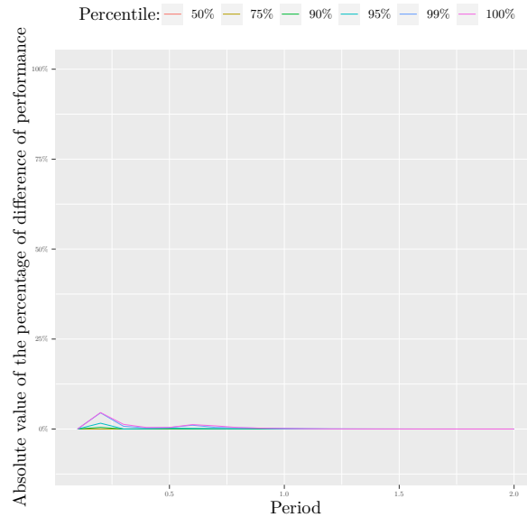
Figure 4.7: Absolute difference in the simulated performance (with 10^6 tasks) of the LMAX+DMAX and NEVERKILL heuristics. For each value of the period \tau , the main percentiles (and worst-case) are presented.
