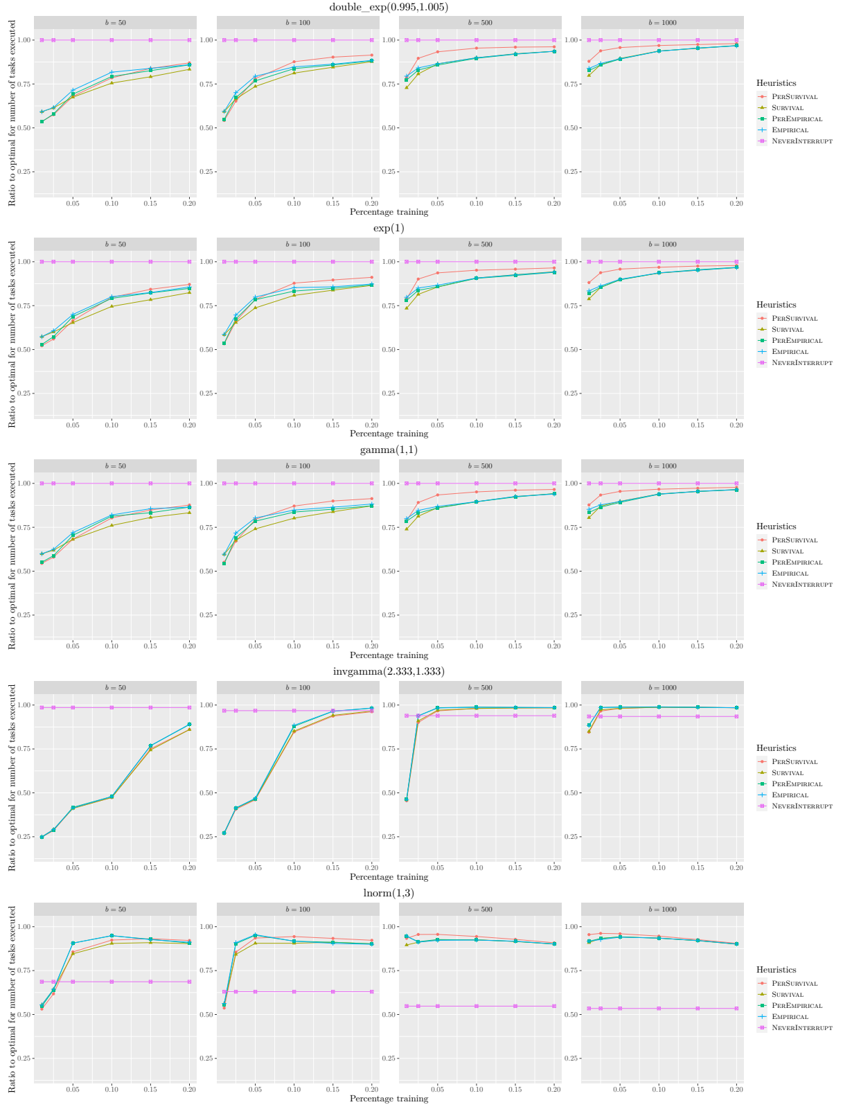
Figure 3.5: Ratio to ORACLE of number of tasks successfully executed using different heuristics when varying p for each distribution (2/3).
