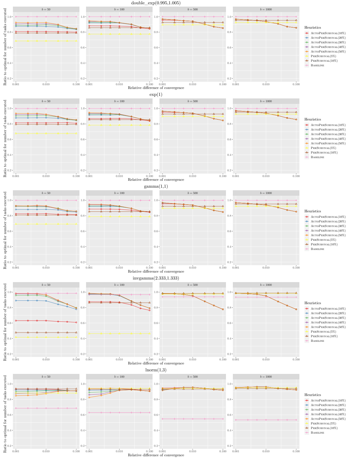
Figure 3.8: Number of successfully executed tasks for each distribution using AUTOBERSURVIVAL (different p_{max} when varying \epsilon ) and PERSURVIVAL (different p ) (2/3).
