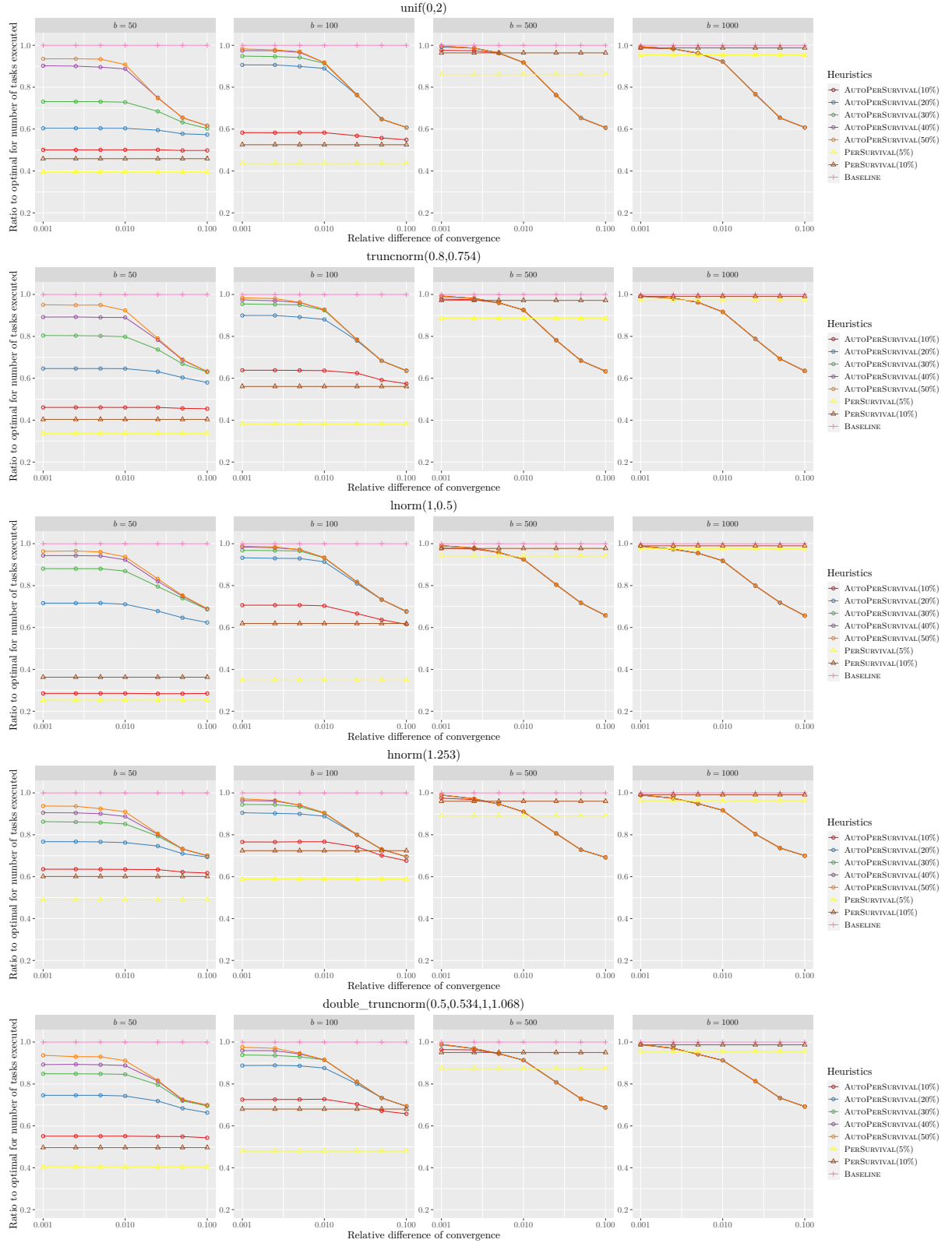
Figure 3.7: Number of successfully executed tasks for each distribution using \text{AUTOPERSURVIVAL} (different p_{\max} when varying \epsilon ) and \text{PERSURVIVAL} (different p ) (1/3).
