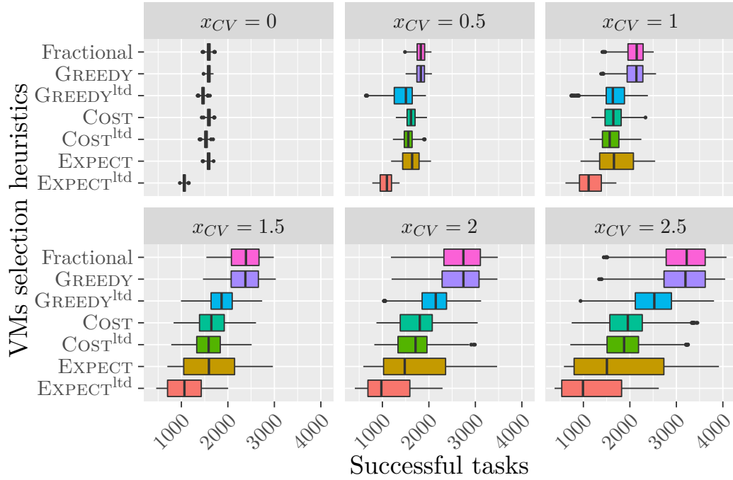
Figure 2.3: Number of successfully executed tasks for resource selection heuristics with OPTRATIO, m_j = 10 , M = 60 , c_j = s_j , b = 630 and d \approx 13.2 . Execution times follow a lognormal distribution with x_{CV} varying.
