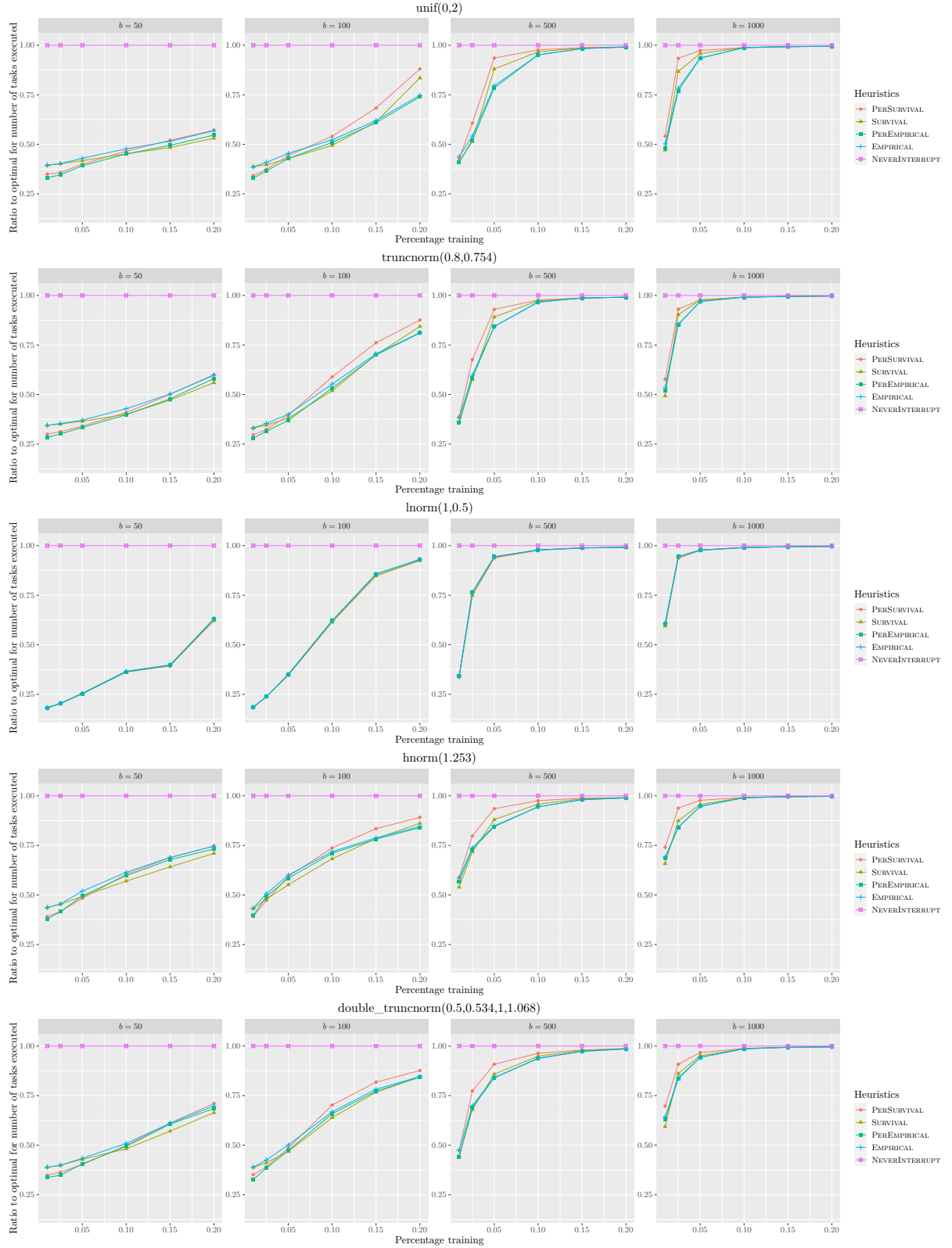
Figure 3.4: Ratio to ORACLE of number of tasks successfully executed using different heuristics when varying p for each distribution (1/3).
