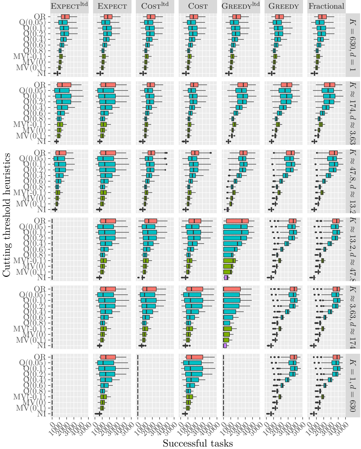
Figure 2.1: Number of successfully executed tasks for different resource selection and cutting threshold heuristics, with m_j = 10 , M = 60 , c_j = s_j , b = 630 . Execution times follow a lognormal distribution with x_{\text{CV}} = 3 .
