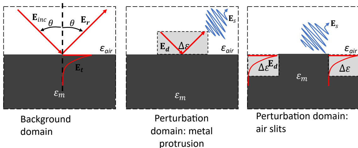
Figure 4.5: Example of a driving field \mathbf{E}_d inside the perturbation domain in the case of a lamellar grating with an absorbing metal substrate with an air superstrate. In (metal protrusion), the driving field inside the perturbation domain is a superposition of the incident and reflected field. In (air slits), the driving field is the transmitted field, exponentially damped inside the metal substrate.
