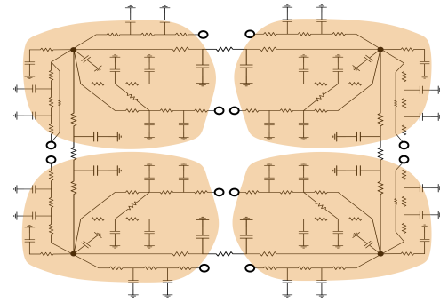
(b) Clustered RC-network model
