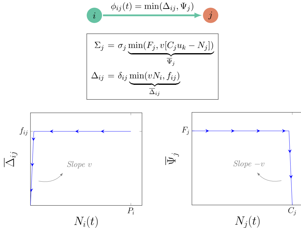
Figure 8.2: An example illustrating the flow \phi_{ij}(t) from origin i to destination j in terms of supply of j and demand of i with respect to j . Here, the arrows on each curve indicate the time evolution.
