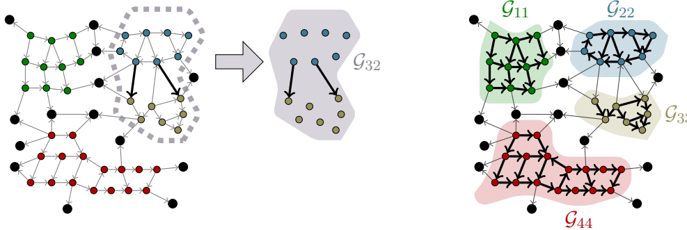
(c) An induced bipartite subgraph \mathcal{G}_{32} capturing inter-cluster topology from cluster \mathcal{C}_2 to cluster \mathcal{C}_3 .
