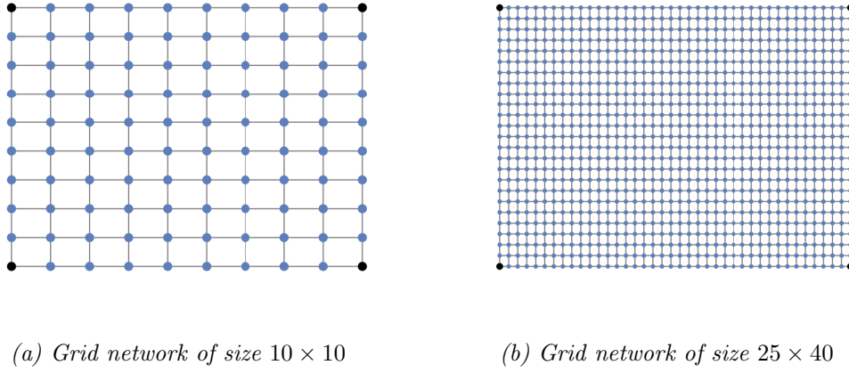
Figure 3.7: Examples of grid networks with four measured nodes (black) at the corners and one cluster of unmeasured nodes (blue).
