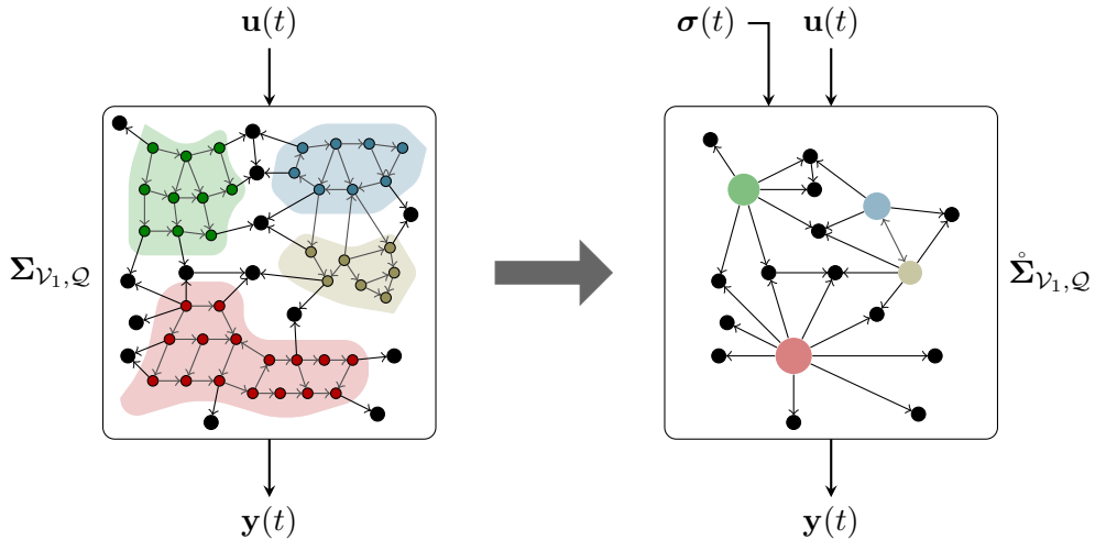
Figure 2.2: Obtaining a projected network system \dot{\Sigma}_{\mathcal{V}_1, Q} from a clustered network system \Sigma_{\mathcal{V}_1, Q} by aggregating the clusters of unmeasured nodes.
