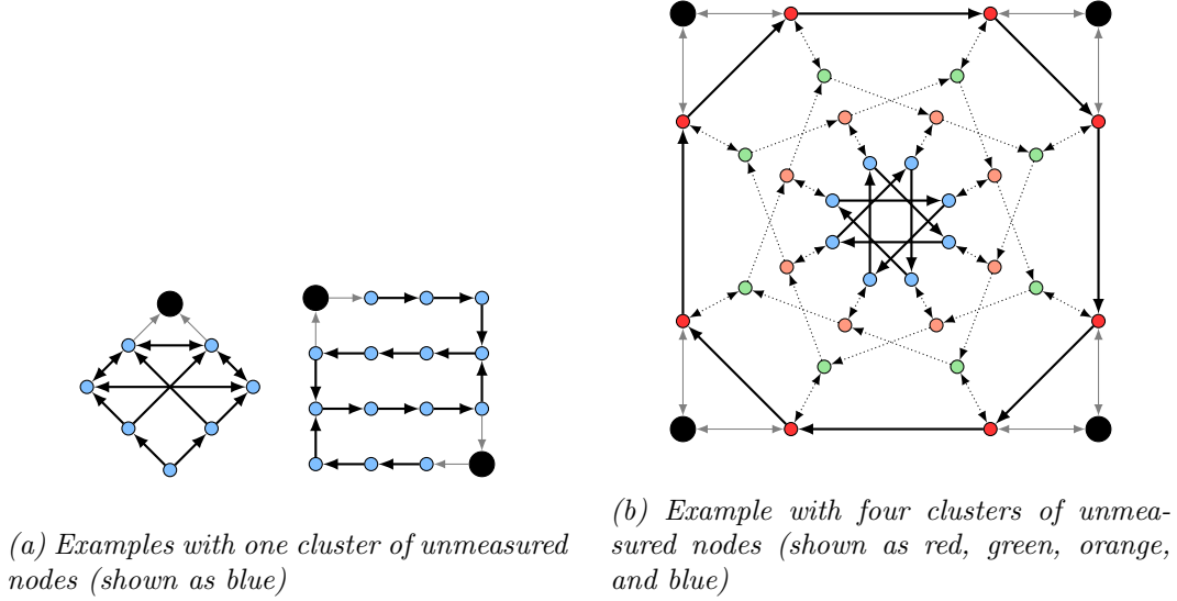
Figure 3.4: Examples of clustered network systems with an equitable clustering of unmeasured nodes.
