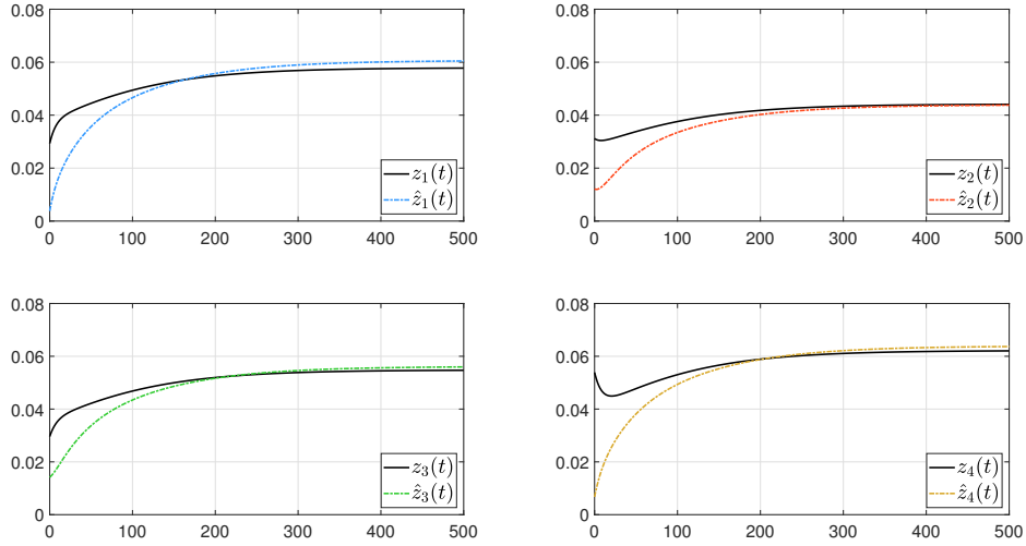
Figure 5.10: Average estimation of four clusters of unmeasured nodes in Figure 5.9.
