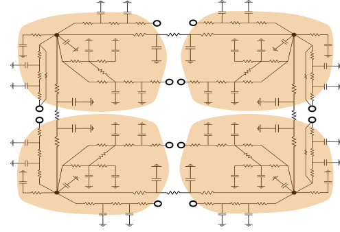
(b) Clustered RC-network model
