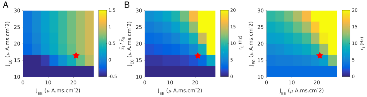
Figure 3-figure supplementary 3. Two-population model. The response of the PC and PV populations upon stimulation of the latter are proportional only if parameters are fine-tuned. A. \frac{\bar{\chi}_I}{\bar{\chi}_E} where \bar{\chi}_\alpha = \frac{\left(\frac{r_{light\ on}}{r_\alpha} - 1\right)}{\Gamma_{opto}} estimated for \Gamma_{opto} = 0.5 mW.mm^{-2} . The ratio is close to one only if J_{EE} \approx J_{EI} \frac{J_{IE}}{J_{II}} = 30 \mu A.ms.cm^{-2} . B. Red star indicates the approximate center of the region with proportionality of the responses together with reasonable activities. Parameters as in Fig. 3. K = 500 .
