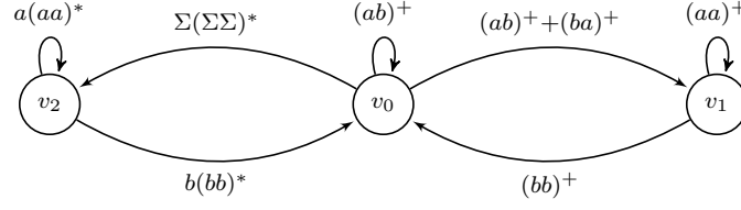
Figure 4.6: Example of a non-deterministic parameterized arena.
