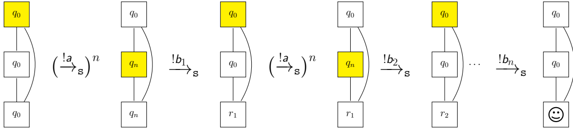
Figure 3.11: A static execution of size 3 and length O(n^2) covering \odot for the protocol of Figure 3.10.
