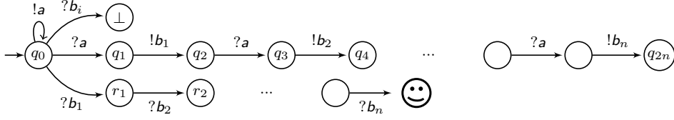
Figure 3.6: Example where reconfigurable semantics needs less nodes than lossy semantics.
