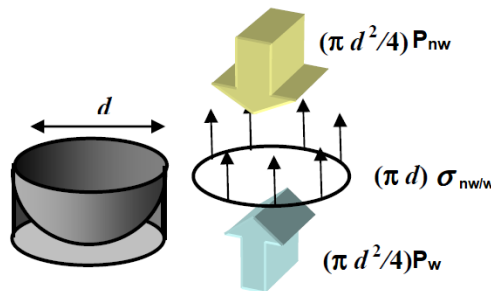
Fig. 2-5 - Laplace Law applied on a spherical meniscus of a pore (Daian, 2013)
