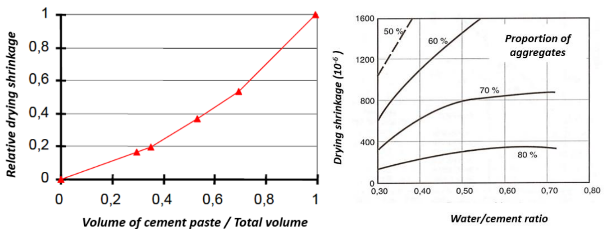
Fig. 4-3 – (left) Relative drying shrinkage strains vs the fraction of cement paste (Benboudjema, 2004) – (right) Drying shrinkage strains vs water/cement ratio (Odman, 1968) cited by Hubert and Giraud (2004)
