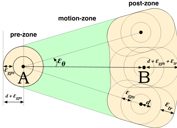
Figure 1.5 – Reservation Zone Given Known Error Upper Bounds
