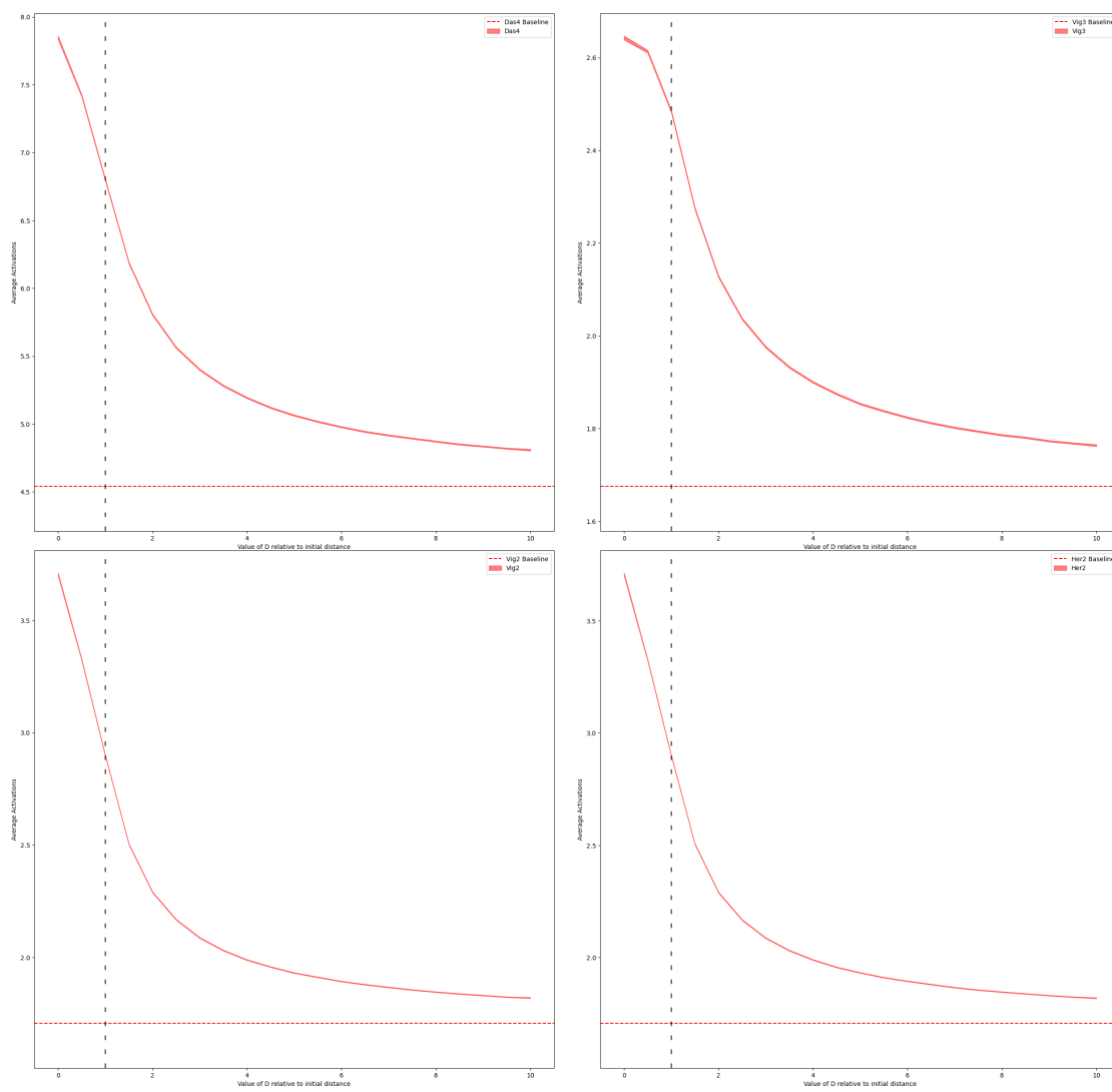
Figure C.8 – Activations for rigid SSYNC
