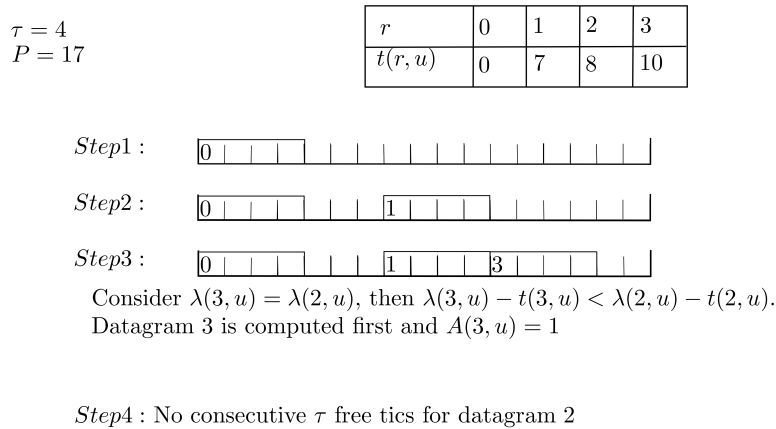
Figure 5.3 – An instance for which Greedy Deadline fails to build an assignment
