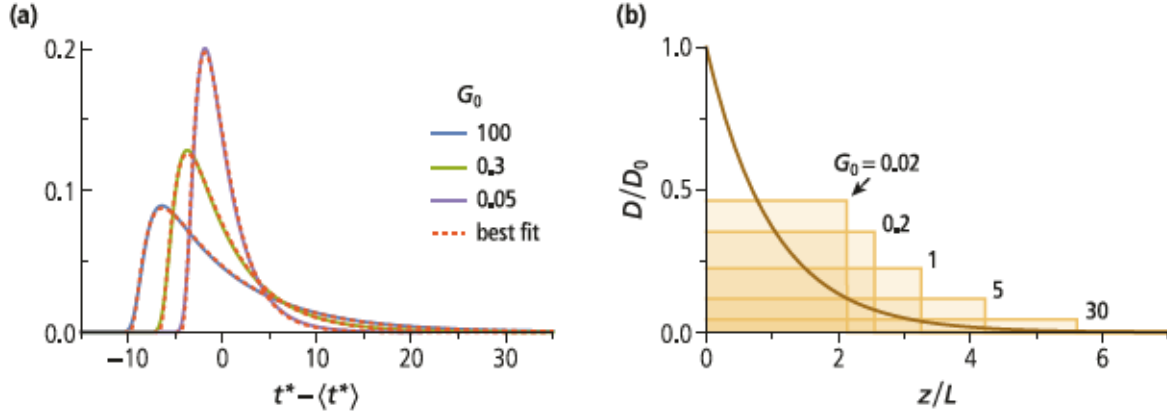
Figure 4.6: (a) Nondimensionalized impulse responses for a mixed layer with exponentially decaying diffusivity (solid lines) and corresponding least-squares fits with rescaled impulse responses for a homogeneous mixed layer, according to eq. (4.18) (dashed lines). The rescaling parameters are (\chi, \omega) = (0.322, 6.653) for G_0 = 100 , (\chi, \omega) = (0.0360, 2.687) for G_0 = 0.3 and (\chi, \omega) = (0.0986, 2.214) for G_0 = 0.05 . (b) Exponential diffusivity profile (brown line) and equivalent homogeneous mixed layers (shaded) for selected values of G_0 . The thickness of the equivalent homogeneous mixed layer increases with increasing G_0 .
