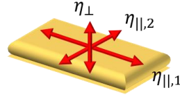
Figure 4-22. 3-dipole model
