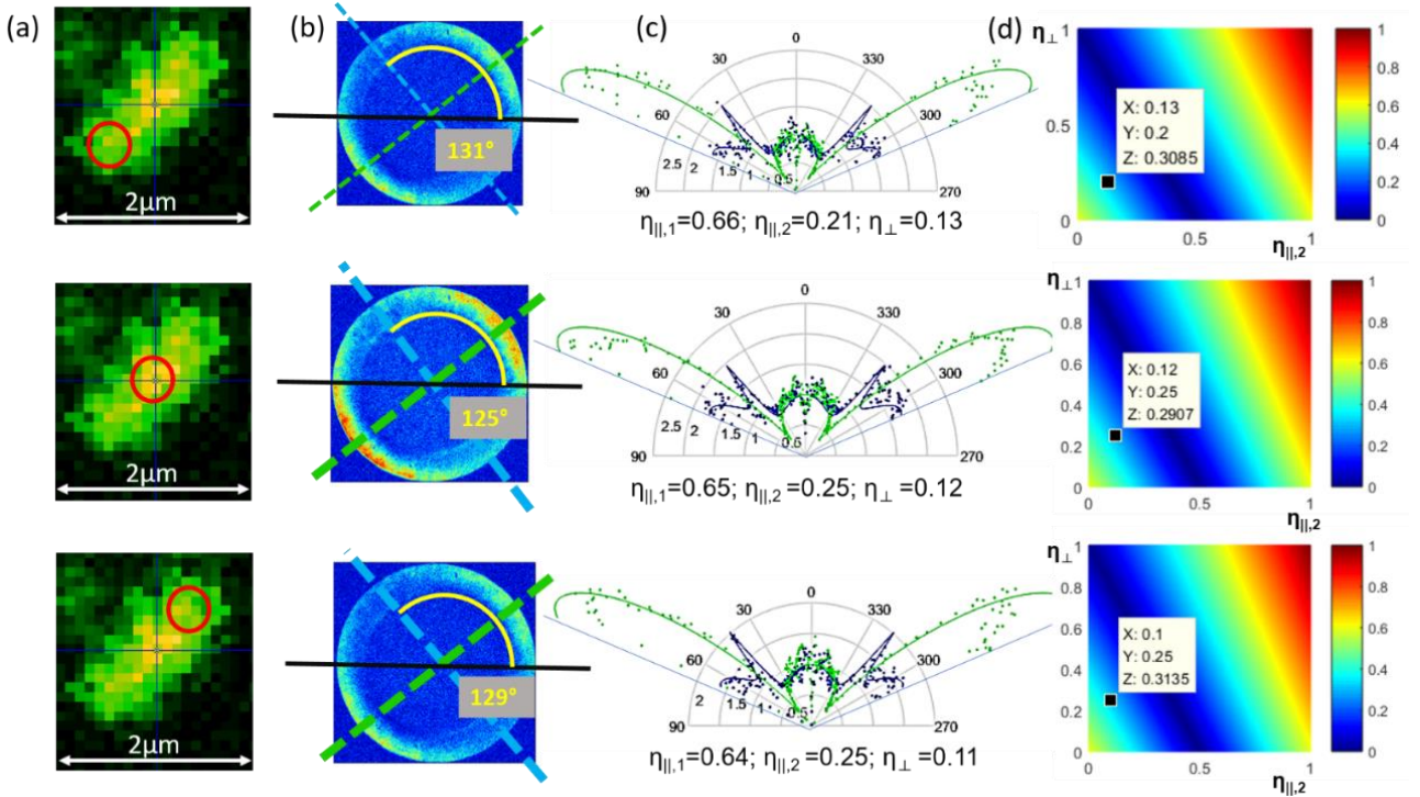
Figure 4-31. Fourier plane image of the same chain. (a) Probe of different portion in the chain. (b) Raw data of Fourier plane image. (c) Fitting (solid lines) of profiles of cutting lines (dots) along two orientations indicated by blue/green dashed lines in Fourier image (c). (d) theoretical degree of polarization \delta_{theo} with dipole portion as extracted in (c).
