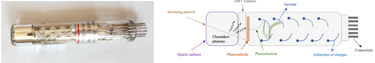
Figure 4.7: Left: a picture of the R760 HAMAMATSU PMT. Right: a schematic view of the PMT amplification chain.
