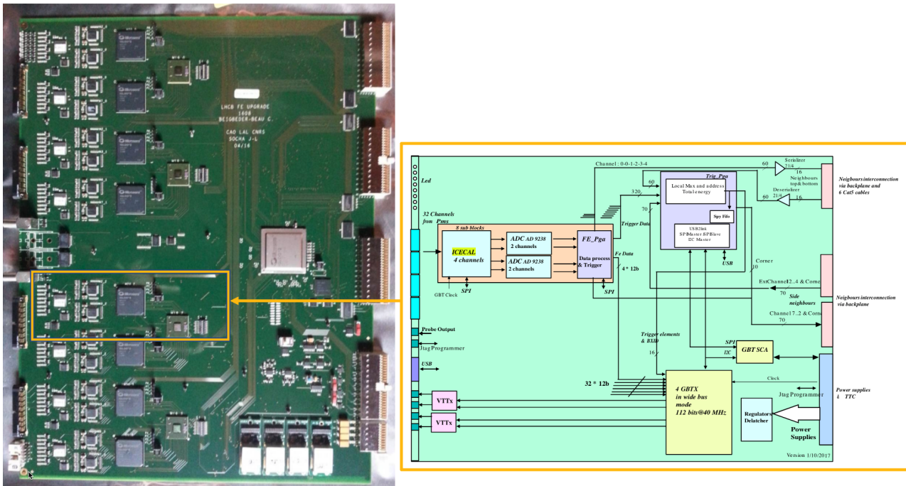
Figure 4.11: Picture of one ECAL FEB with a zoom on the front end block, showing a functional schematics of the front-end block, the power circuitry, the slow control (GBT-SCA) and trigger module, adapted from [193].
