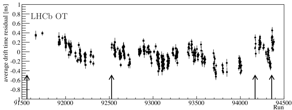
Figure 4.14: Average drift time residuals measured by the LHCb OT. Every point is a one hour run. The arrows show the adjustment of the LHCb clock, from [197].
