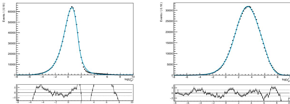
Figure 6.4: Fit of the \log(\chi_{\text{IP}}^2) simulated MC distributions for prompt (left) and secondary (right) produced \Lambda_c^+ .
